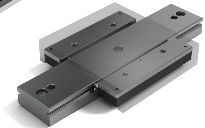
Application with recirculating units and a linear guideway of type RD
