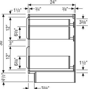
TWO-DRAWER BASE CABINET with ROLL TRAY
