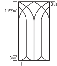
Widths > 11" 3 Vertical Bars Equally Spaced
