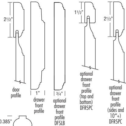
Optional Drawer Front: Raised 5-Piece (DFR5PC)
