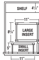
FRONT OF CABINET DOOR HINGED LEFT
