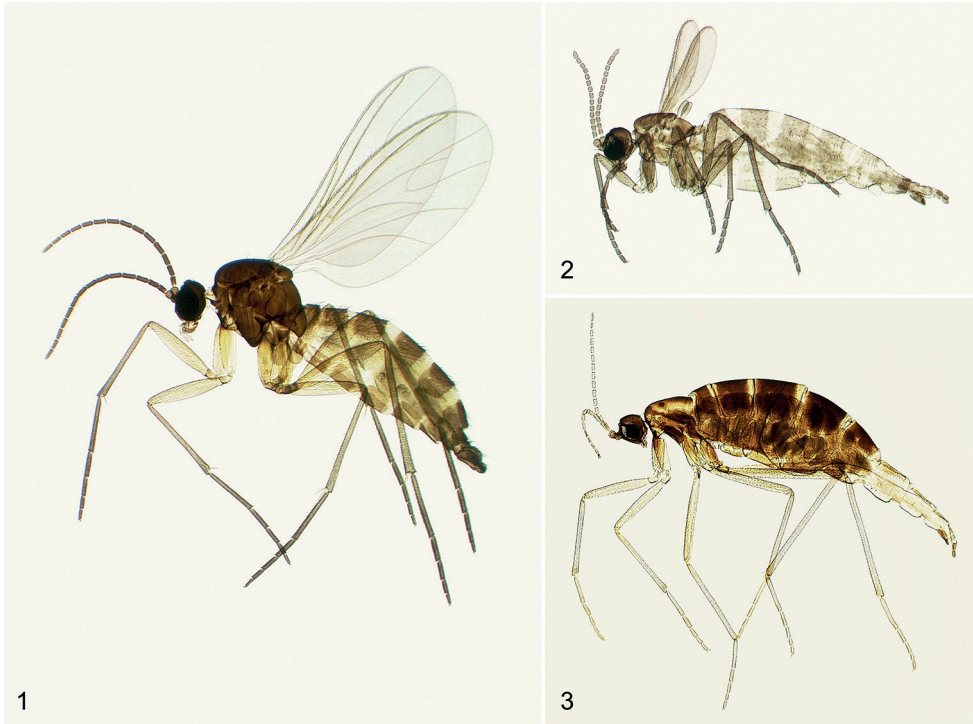
Figures 1–3. Habitus of Norwegian Sciaridae 1 winged male of Bradysia fenestralis (Zetterstedt, 1838) 2 brachypterous female of Corynoptera minima (Meigen, 1818) 3 apterous female of Epidapus gracilis (Walker, 1848).
