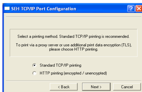
Fig. 9: SEH Print Monitor – Selecting a Printing Method
