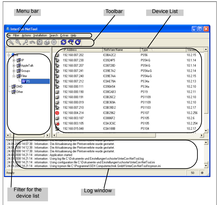
Fig. 3: InterCon-NetTool - Main Dialog
