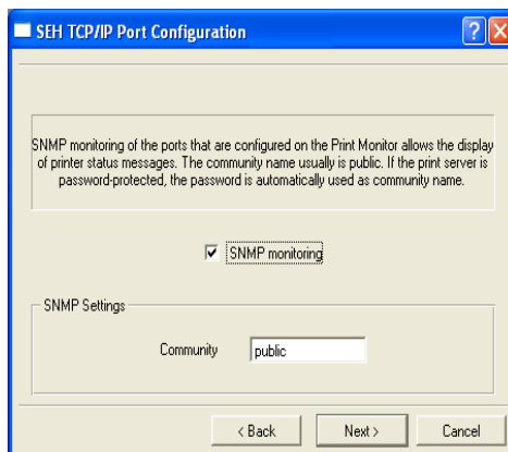
Fig. 11: SEH Print Monitor - SNMP
