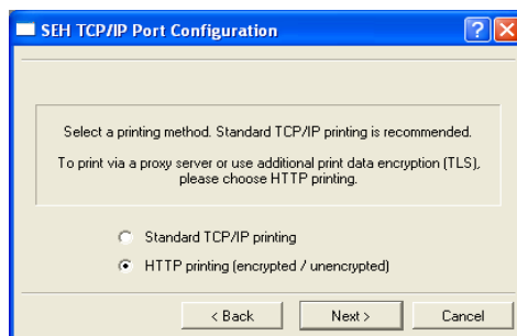
Fig. 12: SEH Print Monitor – Selecting a Printing Method
