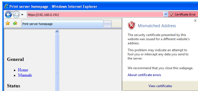
Fig. 48: Internet Explorer
