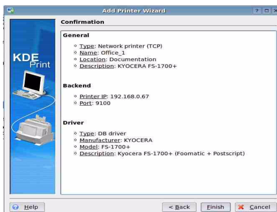
Fig. 34: Add Printer Wizard - Confirmation
