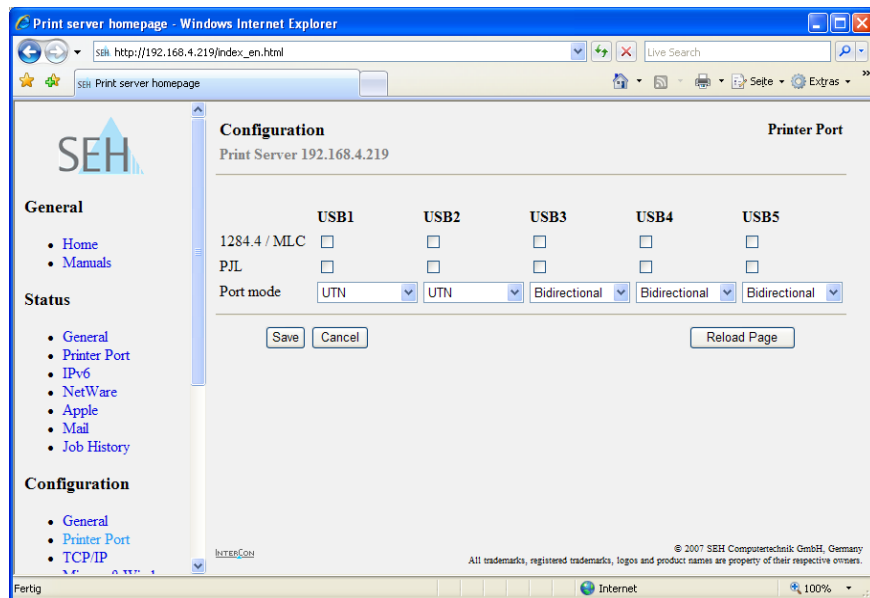
Fig. 60: Print Server Homepage – Printer Port
