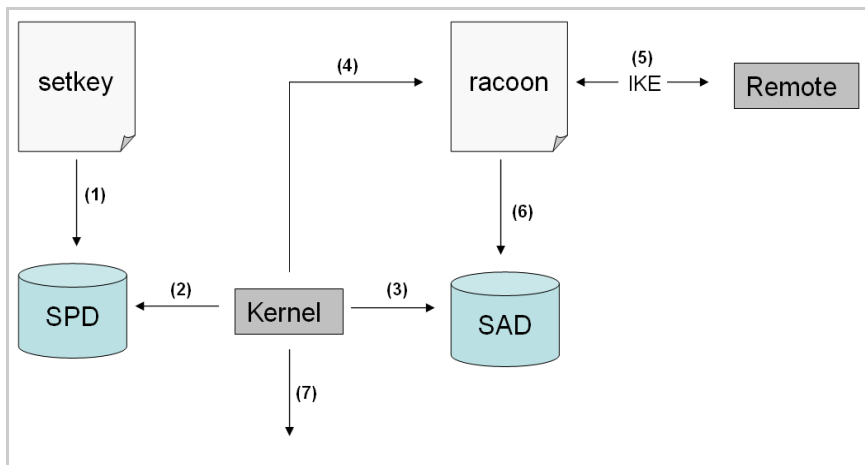
Fig. 50: IPsec procedure
