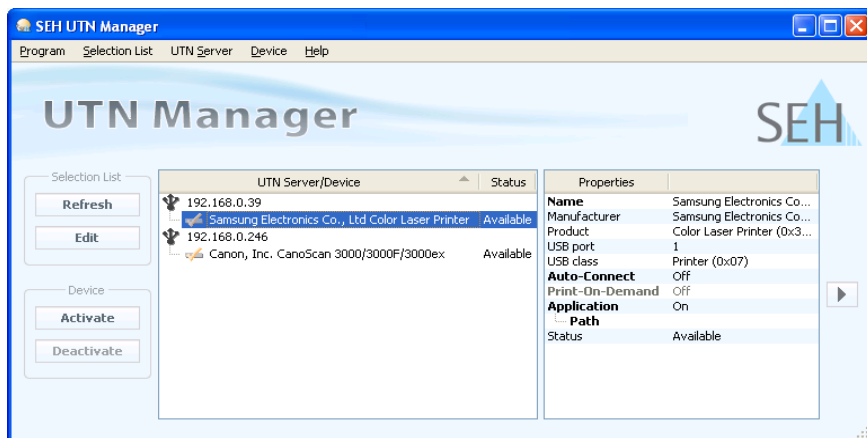
Fig. 61: SEH UTN Manager - Main Dialog
