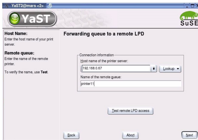
Fig. 22: YaST Control Center - Forwarding queue to a ...
