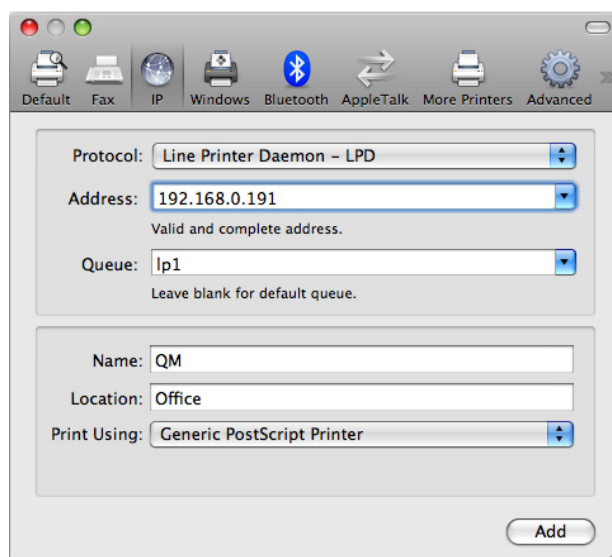
Fig. 16: Mac OS - LPD Printer Installation
