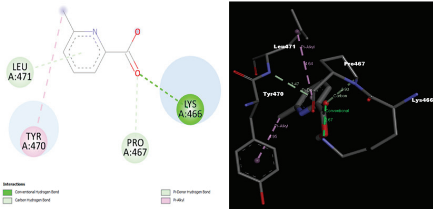
Figure 3: 2D and 3D Structures Showing the Interactions Between \alpha -Glucosidase and 6-Methylpicolinic Acid
