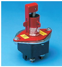
BOSCH DOUBLE POLE ISOLATOR ASSEMBLY PN:844112
