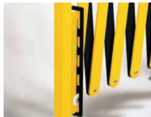
FIXED POSITION LOCKING BAR Locking in 5 different positions: 1 metre; 2 metres; 2.5 metres; 3 metres or fully extended at 3.5 metres. Suitable for Super-Guard & Flexi-Guard models only. PN: HS7091
