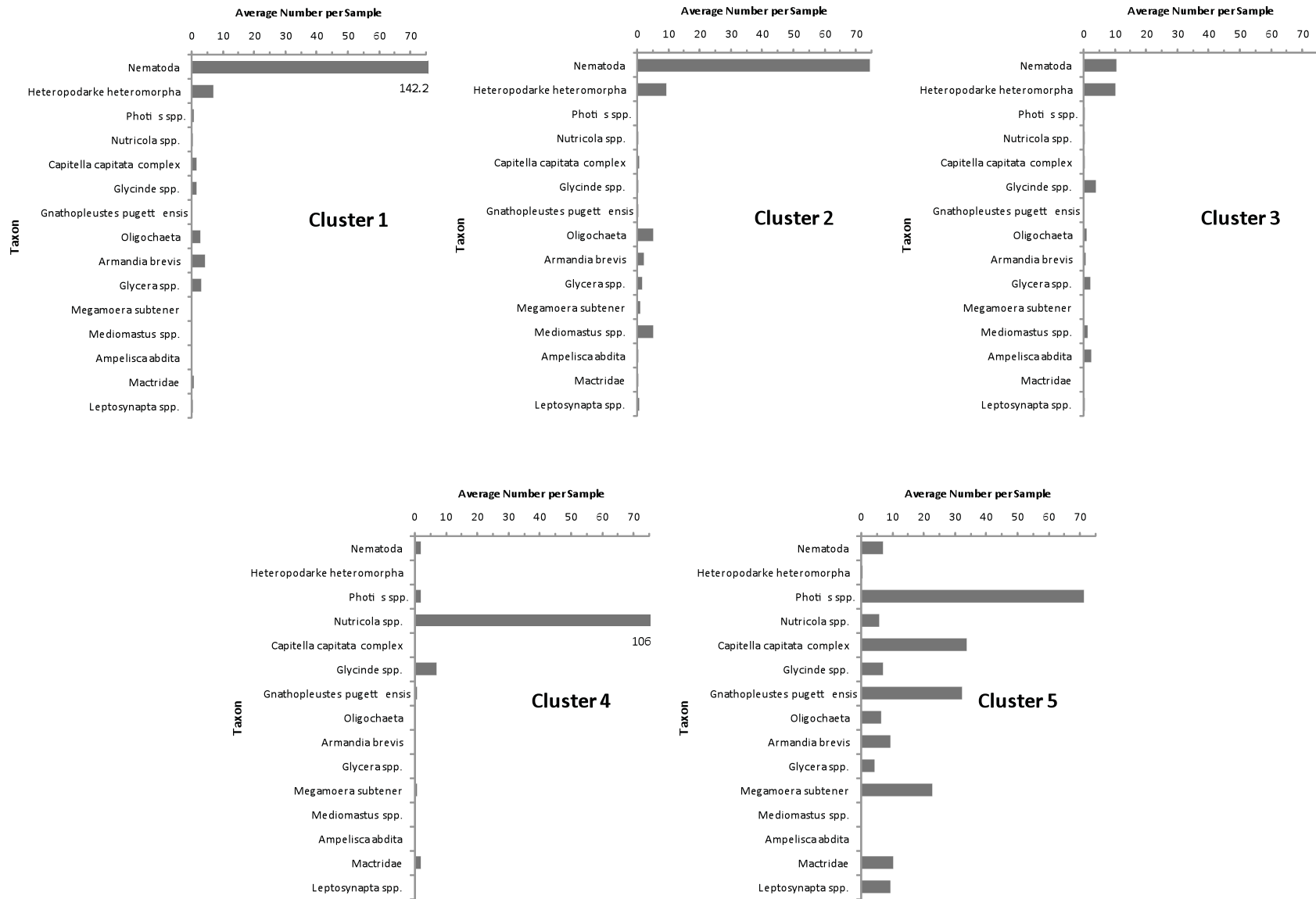
Figure 3-2. Densities of the 15 most abundant benthic taxa in five clusters identified for Central Bay sites
