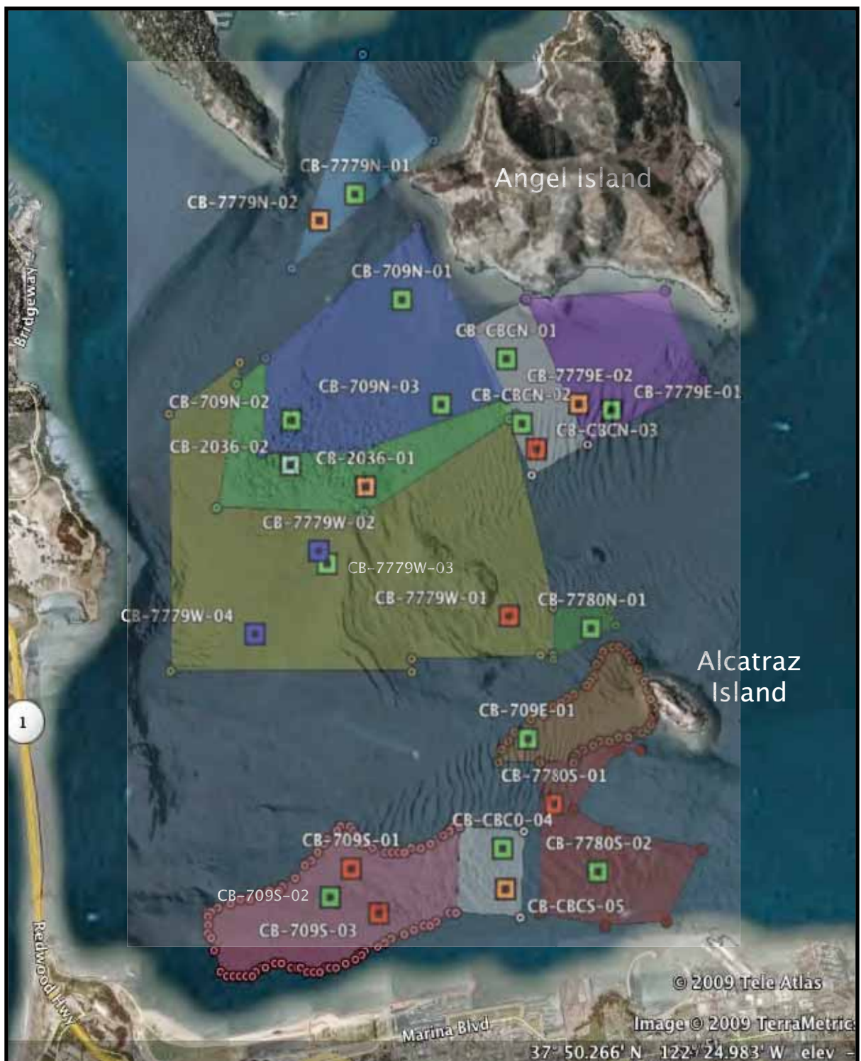
Figure 3-4. Overlay of survey station locations (squares) relative to standing sand waves and other seafloor microhabitats in Central Bay. Colors of square site symbols correspond to clusters in Figure 3-1.
