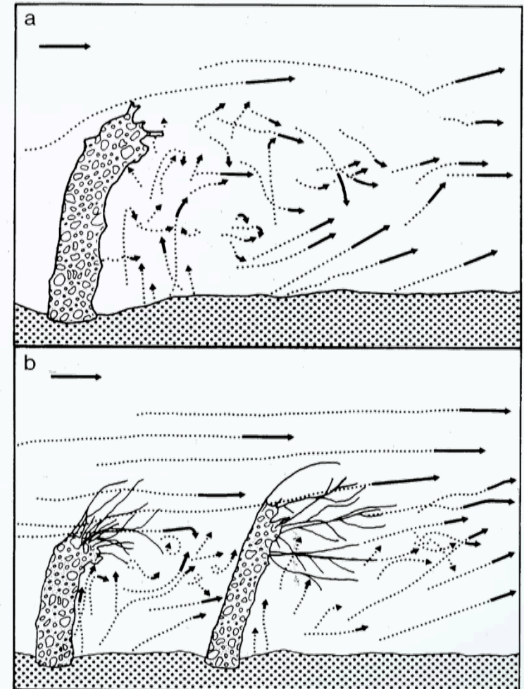
FIG. 3. Velocities of egg particles resuspended in the wake envelopes of Lanice conchilega tubes, measured from pathlines on flume photographs. Vector length represents length of pathlines relative to mean length of undisturbed pathlines calculated for each photograph. Lengths of pathlines are equivalent to time averaged velocities of particles. Reference vector (100% of channel flow velocity) in upper left. Dot lines are observed pathlines. Channel flow velocity 10-11 \text{ cm} \cdot \text{s}^{-1} in all photographs. (a) Adult tube, built in tank, fringe not present. Summary of eight photographs ( \frac{1}{8} to \frac{1}{2} s exposure). Mean percentage of channel flow velocity of particles within wake envelope is 35.08 \pm 6.27 (at 95% confidence level, n = 46 ). (b) Adult tubes, natural spacing, orientation and fringes. Summary of six photographs ( \frac{1}{8} to \frac{1}{2} s). Mean percentage of channel flow velocity of particles within wake envelopes is 31.47 \pm 7.64 (95% CL, n = 30 ). Tubes are 0.5 cm wide.
