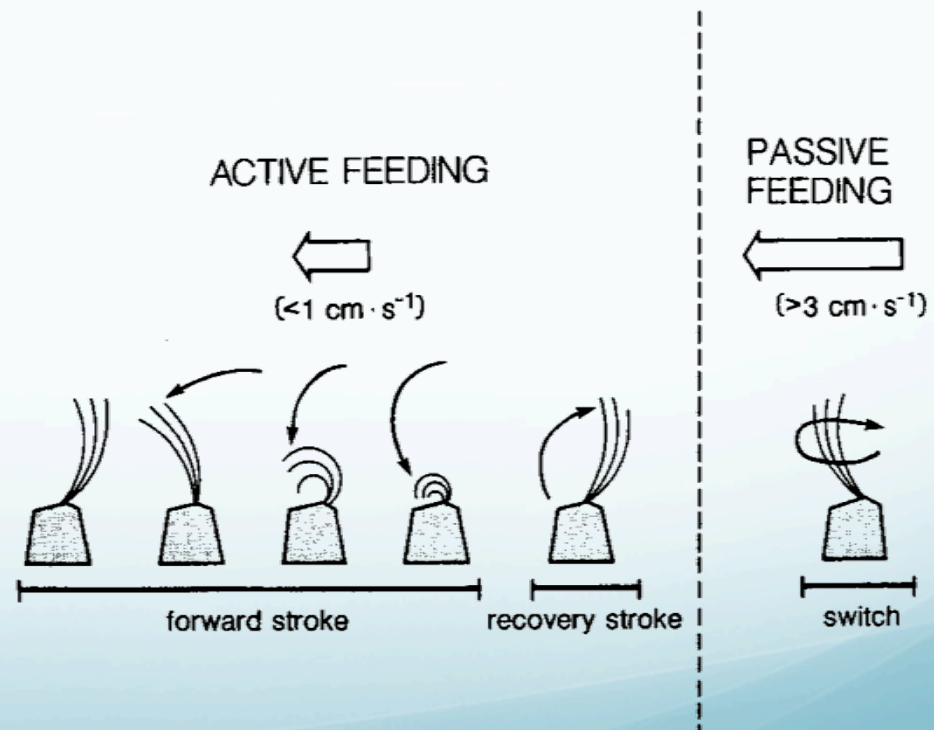
Figure 4.11 Active and passive feeding in Semibalanus balanoides (Trager et al. 1990).
