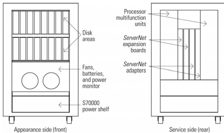
Inside view of components within a NonStop S-series enclosure.
