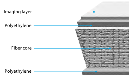
Cross section of an HP photo paper
