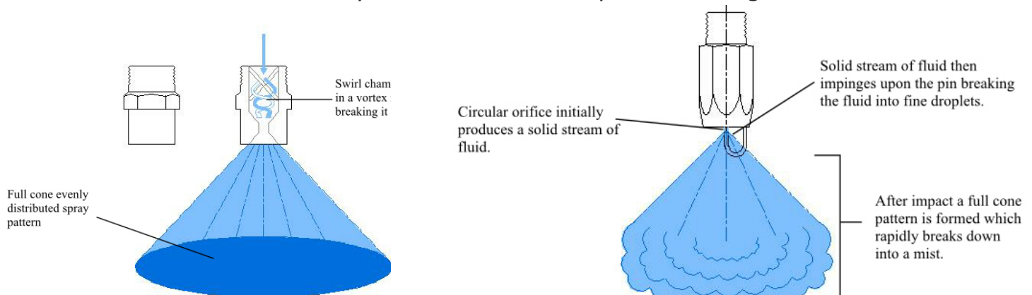
Axial whirl full cone nozzle
