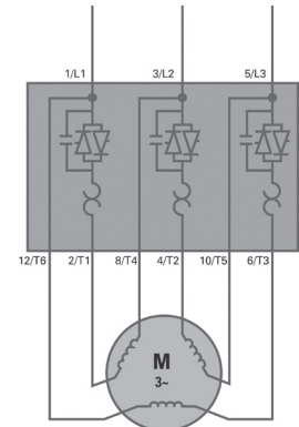
Delta Connected
