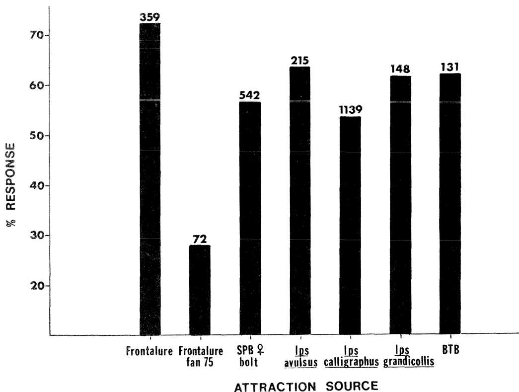
Figure 21.—Wind tunnel responses with frontalure, bolts infested with female SPB, male Ips avulsus , I. calligraphus or I. grandicollis , or field collected bolts infested with Dendroctonus terebrans (BTB) placed in the upwind compartment. (Fan 75 indicates increased wind speed. Numbers are total of beetles tested.)
