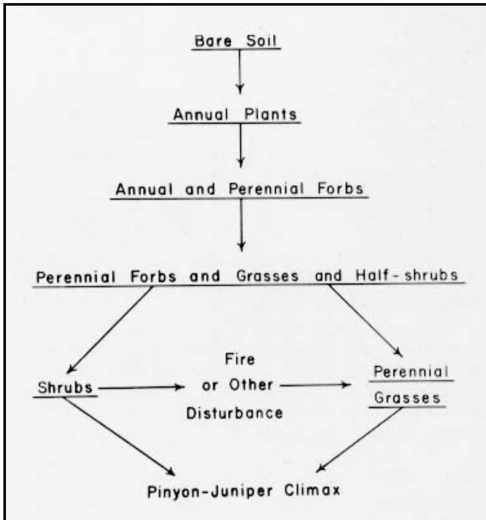
Figure 1- Possible series and pathways of secondary succession following disturbance in pinyon-juniper woodlands (3).
