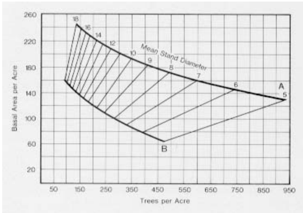
Figure 2- Stocking guide for nearly pure even-aged white pine stands, showing basal area per acre, number of trees per acre, and mean d.b.h. for trees in the main crown canopy (55).
