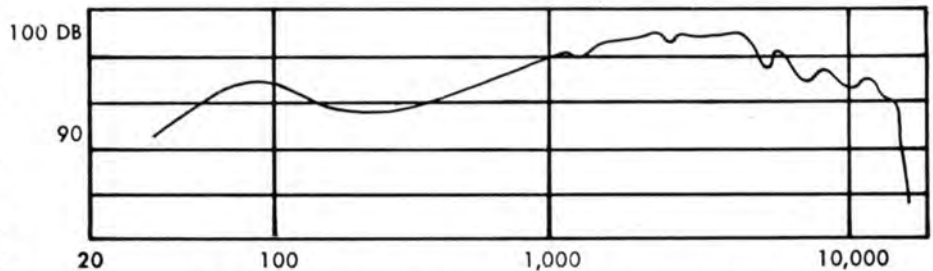
TYPICAL RESPONSE ON CENTER LINE (4 ft.-ONE WATT)
