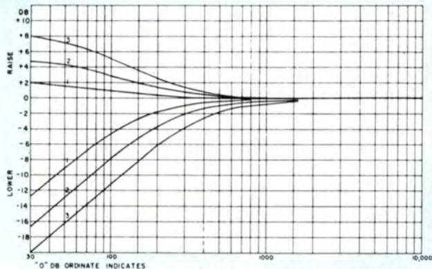
Frequency Response MI-10413.
