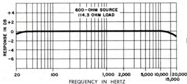
Frequency Response Curve, MI-9289-B Power Amplifier
