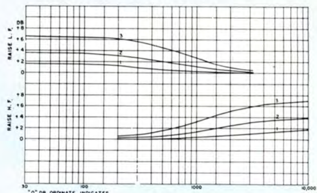
Frequency Response MI-10414.
