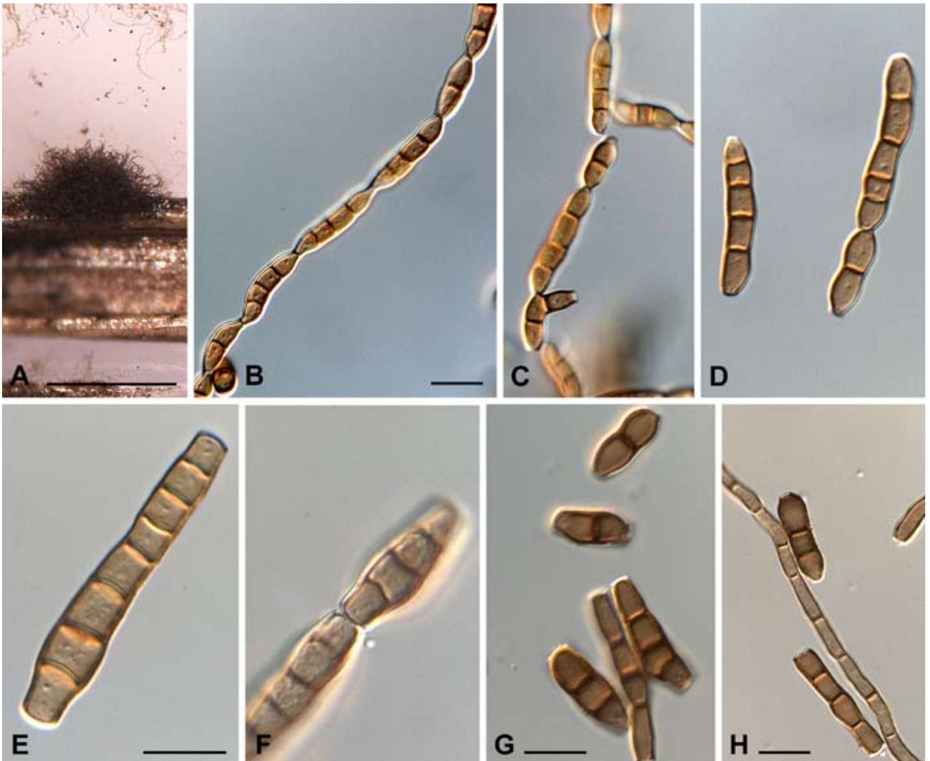
Fig. 6. Catenulostroma chromoblastomycosum (type material). A. Sporodochium on pine needle in vitro . B–H. Chains of disarticulating conidia. Scale bars: A = 350, B, E, G, H = 10 μm.
