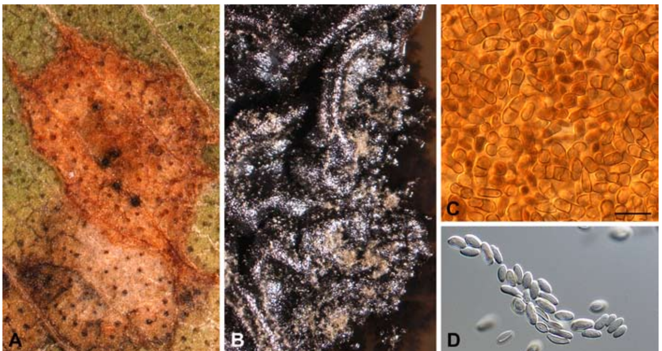
Fig. 19. Readeriella brunneotingens (type material). A. Leaf spot. B. Colony on MEA. C–D. Conidia. Scale bar = 10 \mu m.
