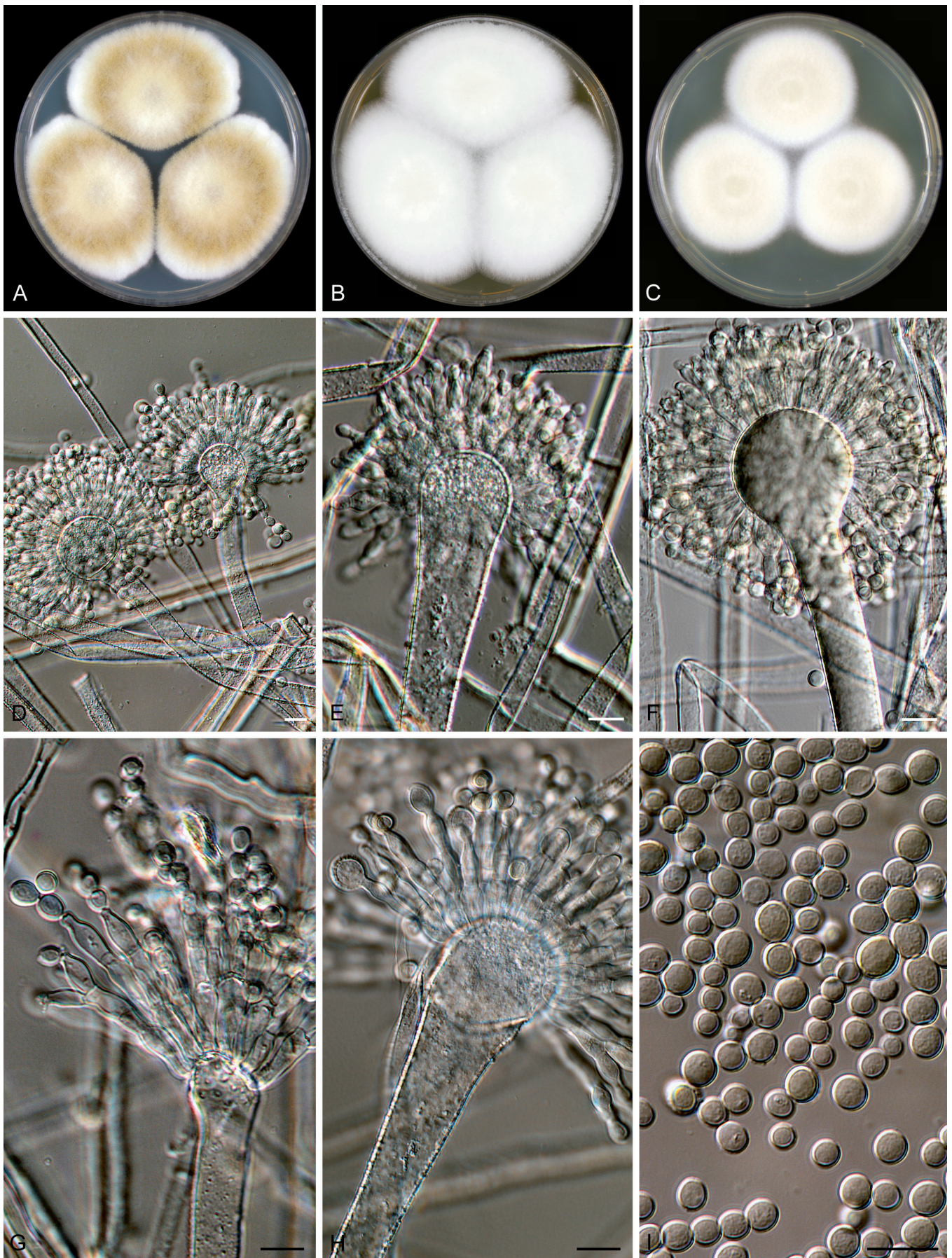
Fig. 16. Aspergillus oryzae (ex-type CBS 100925). A–C. Colonies incubated at 25 °C for 7 d, A. CYA, B. MEA, C. YES, D–I. Conidiophores and conidia. Scale bars = 10 \mu m.
