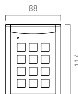
Codeschloss AZF50000-0010
