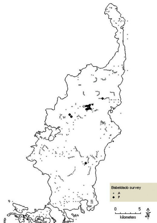
Total distribution of Parkia in Palau, primarily restricted to one population.
