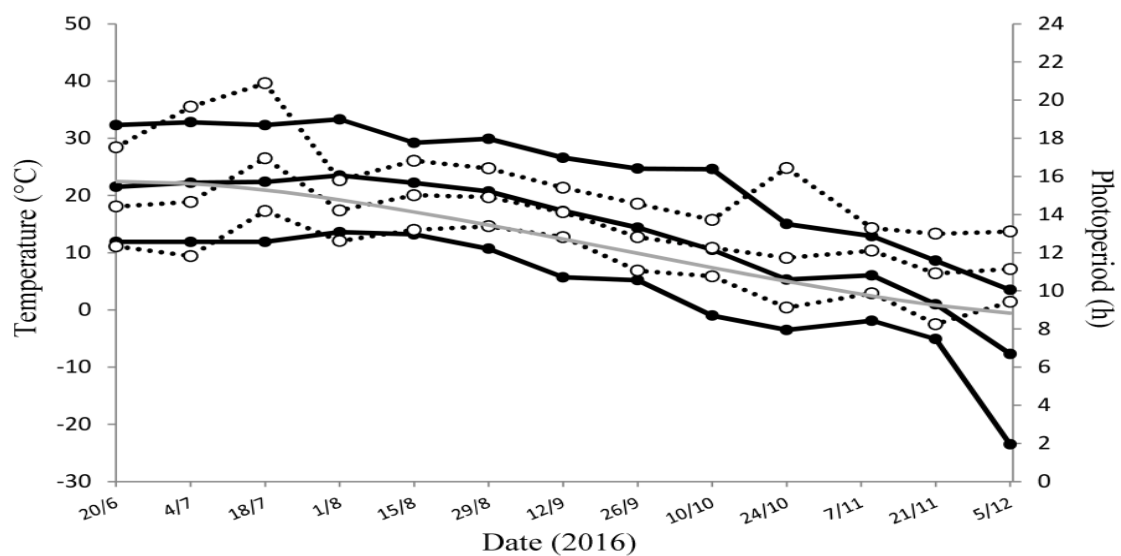
Figure 5.1: Minimum, mean and maximum temperatures (°C) in Montréal, QC, Canada (solid lines) and Rennes, Brittany, France (dotted lines) from 20 th June to 5 th December, 2016. Data shown at each date is the average of temperature data for the 14 days following this date. Photoperiod at 46.50°N is shown for each date (grey line).
