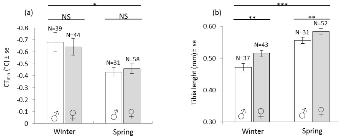
Figure 11.3: Average critical minimal temperature (a) and average tibia length (b) for A. rhopalosiphii in winter and spring. N=172 for CT min measurements and 163 for size measurements. Symbols indicate parasitoids sexes males (♂) and females (♀). *** p<0.001 ** p<0.01 * p<0.05 n.s.=not significant.
