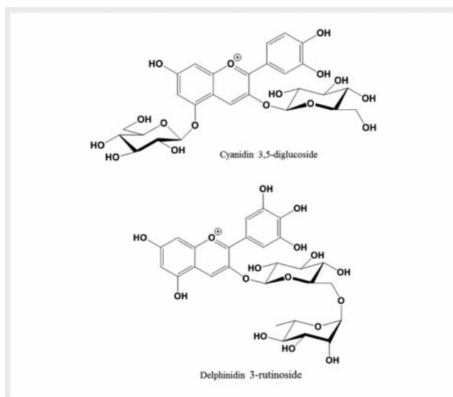
► Fig. 3 Chemical structure of cyanidin 3,5-digluco- \beta -D-glucopyranoside and delphinidin 3-rutinoside.
