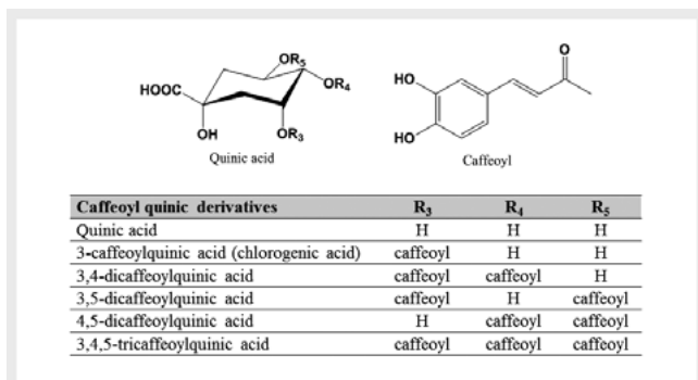
► Fig. 6 Chemical structures of caffeoylquinic derivatives from I. batatas leaves [67].
