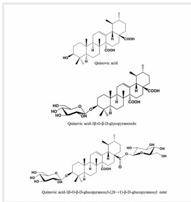
► Fig. 2 Chemical structure of quinovic acid, quinovic acid-3 \beta -O- \beta -D-glycopyranoside, and quinovic acid-3 \beta -O- \beta -D-glucopyranosyl-(28 \rightarrow 1)- \beta -D-glucopyranosyl ester.
