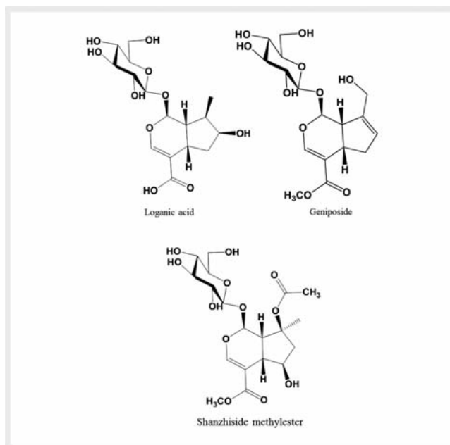
► Fig. 5 Chemical structures of loganic acid, geniposide, and shanzhiside methylester.
