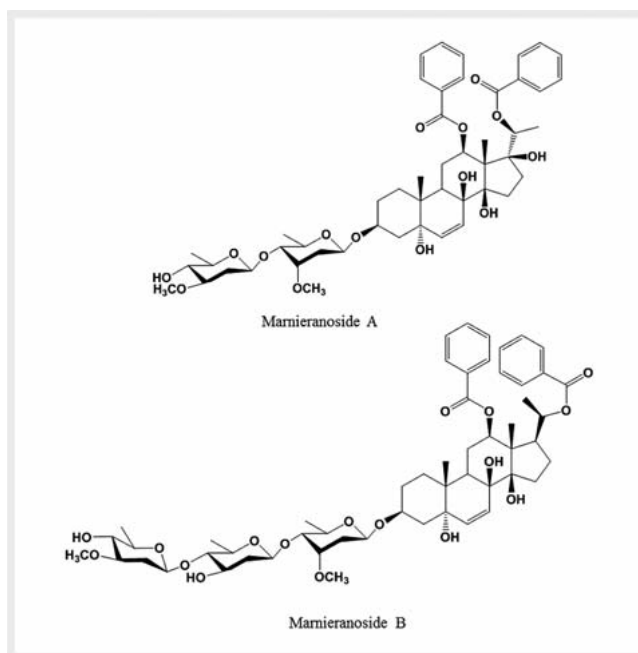
► Fig. 4 Chemical structure of marnieranosides A and B.
