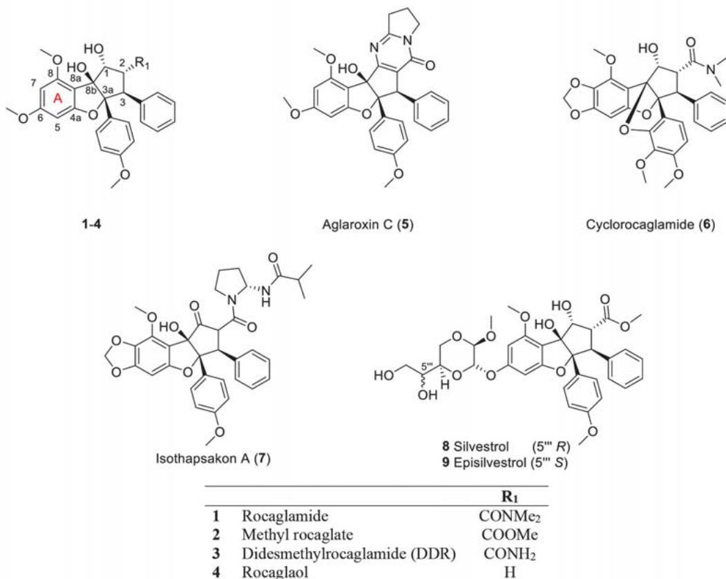
► Fig. 1 Examples of selected flavaglines (1–9) isolated from various Aglaia species.
