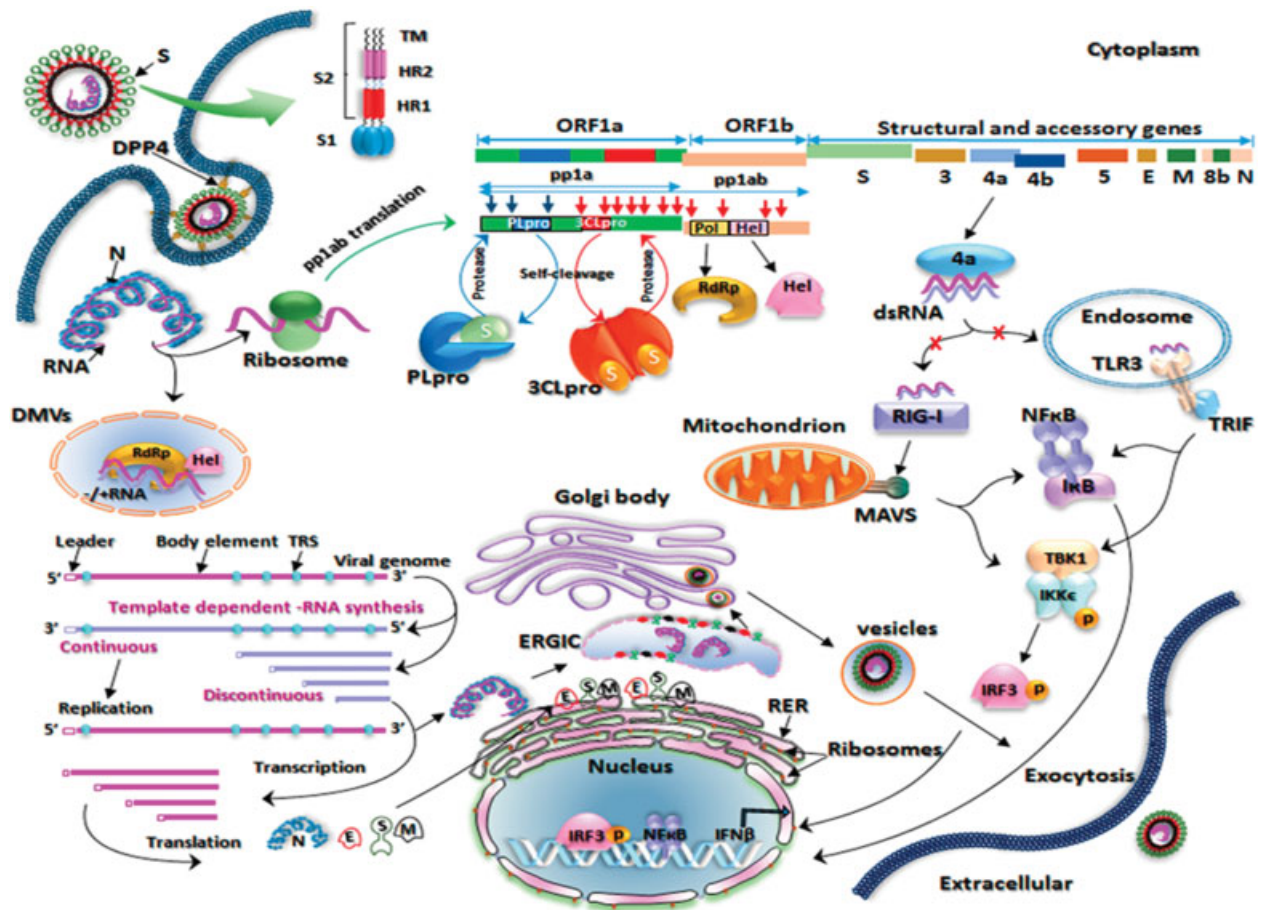
Fig. 1 Schematic of the replication cycle of Middle East respiratory syndrome coronavirus (MERS-CoV). MERS-CoV binds to dipeptidyl peptidase 4 (DPP4) on the host cell through its receptor-binding domain (RBD) in the S1 subunit of the spike (S) glycoprotein, which leads to virus–cell fusion and the release of genomic RNA into the cytoplasm. Initially open reading frame 1a (ORF-1a) and ORF-1b are translated into polyproteins, polyprotein 1a (pp1a) and pp1ab, respectively, which are cleaved by the virus-encoded proteases papain-like protease (PLpro) and 3C-like protease (3CLpro) into 16 mature nonstructural proteins (nsps). The proteins involved in replication and transcription are gathered into replication-transcription complexes (RTCs) that associate with double-membrane vesicles (DMVs) derived from the endoplasmic reticulum (ER). The genomic RNA contains adenylate uridylylate (AU)-rich sequences called transcription regulation sequences (TRSs). If the TRSs are recognized by RTCs, then RNA of subgenomic length for transcription will be generated, otherwise a full-length template RNA of genomic length for replication will be synthesized. The newly produced genomic RNAs are encapsidated in the nucleocapsid (N) proteins in the cytoplasm and then transported to the ER–Golgi intermediate compartment (ERGIC) for further assembly. The S, membrane (M), and envelope (E) proteins are inserted into the membrane of the rough ER (RER), from where they are transported to the ERGIC to interact with the RNA-encapsidated N proteins and assemble into viral particles. The budded vesicles containing mature viral particles are then transported to the cell surface for release after maturation in the Golgi bodies. Double-stranded RNAs (dsRNAs) are partially generated during viral replication. The 4a competes with Toll-like receptor 3 (TLR3) and retinoic acid-inducible gene I product (RIG-I)-like helicases (RIG-I and melanoma differentiation-associated protein 5 [MDA5]) to bind to dsRNAs and evades the host immune response. (Adapted from Durai P, Batool M, Shah M, Choi S., Middle East respiratory syndrome coronavirus: transmission, virology and therapeutic targeting to aid in outbreak control. Exp Mol Med 2015;47:e181; doi:10.1038/emmm.2015.76 under Creative Commons CC-BY license (Creative Commons Attribution 4.0 International License). 2
