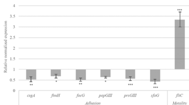
► Fig. 1: Relative gene expression of selected virulence factors (VF) from E. coli strain UTI89 determined by Illumina RNA-Seq. considering the effects of OWE oPC [2 mg/mL] on VFs regulations after 2 h incubation in urine. All the expressions are related to untreated control adjusted at one.
