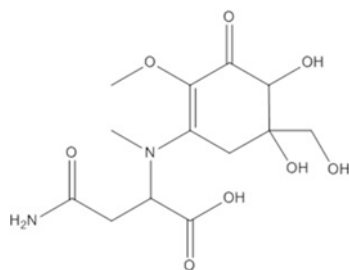
► Fig. 1: N 2 -(4,5-dihydroxy-5-(hydroxymethyl)-2-methoxy-3-oxocyclohex-1-en-1-yl)-N 2 -methylasparagine
