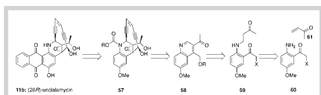
Fig. 16 Retrosynthetic approach developed by P. van de Weghe and colleagues.
