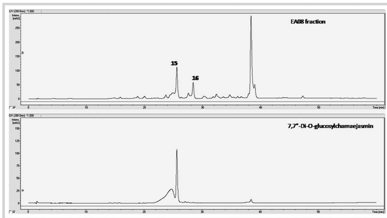
Fig. 5 HPLC profile of fraction EA08 of Ormocarpum kirkii compared to the chromatogram of 7,7''-di- O - \beta -D-glucosylchamaejasmin using 0.05% TFA in water (A) and MeOH (B): 0 min, 80:20 (A:B); 20 min, 60:40; 30 min, 57:43;
