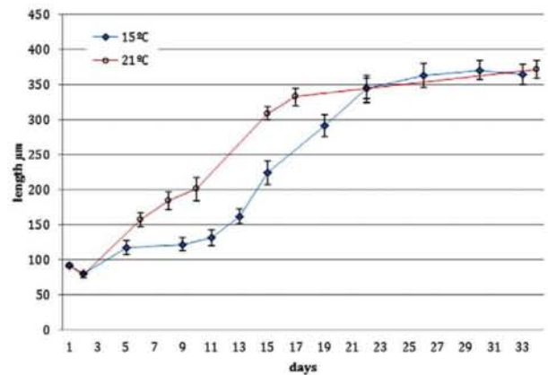
Fig. 8. – Sabellaria spinulosa . Larval growth rate at 15°C and 21°C.
