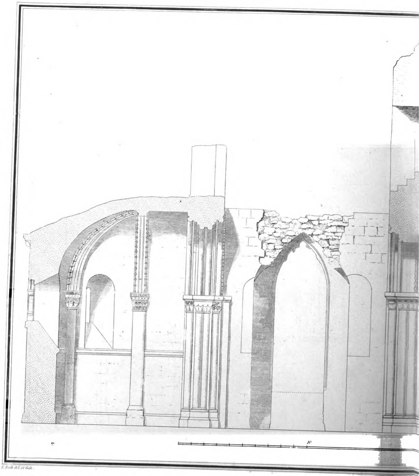
Section of Steetley Church
