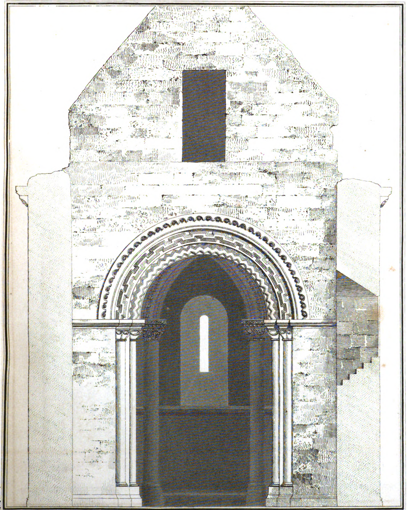
Transverse Section of Steetley Church Digitized by Google
