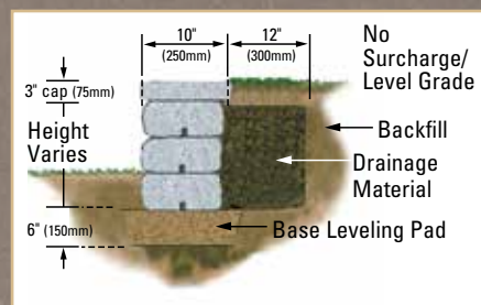
GRAVITY WALL Setback Detail 9.5° ± Batter
