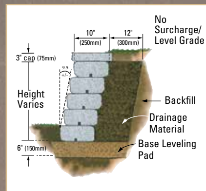
GRAVITY WALL Setback Detail 9.5° ± Batter
