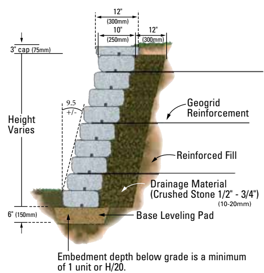
REINFORCED WALL Setback Detail 9.5° ± Batter
