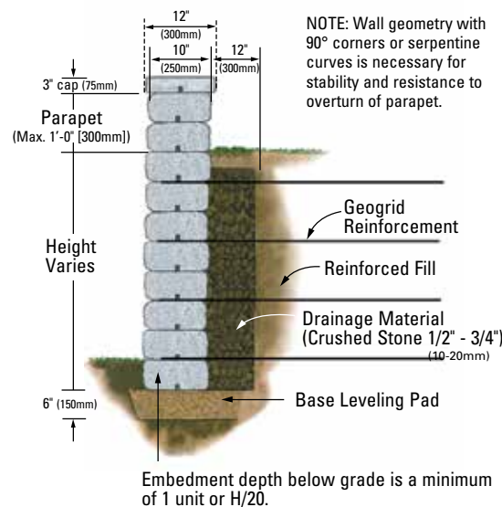
REINFORCED WALL Near Vertical Detail
