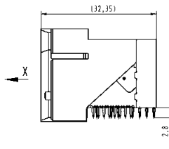
view X
