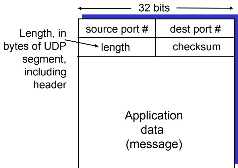
UDP segment format
