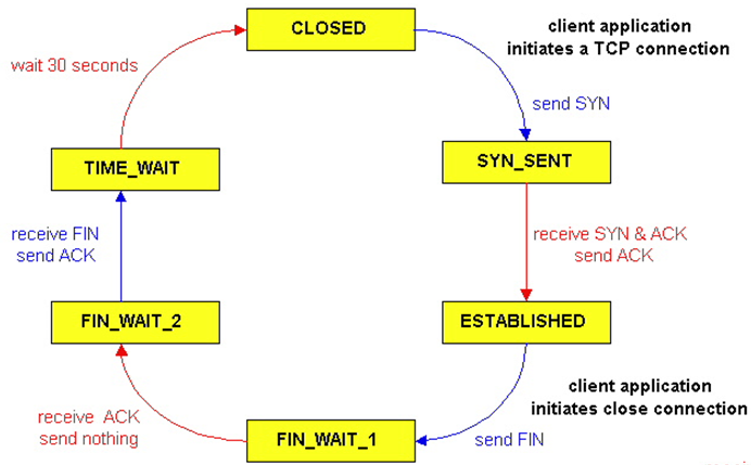
TCP Client Lifecycle
