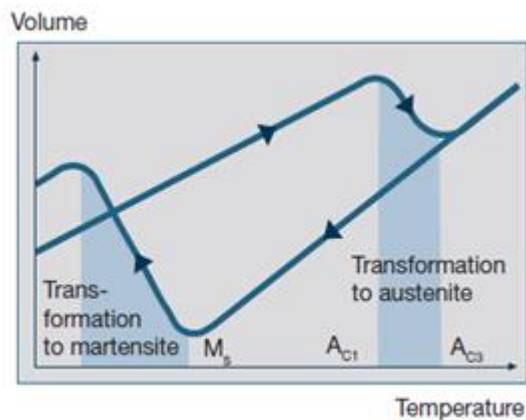
Fig. 1 Volume changes due to structural transformation
