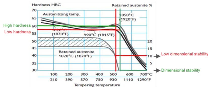
Fig. 3. Dimensional stability AISI D2
