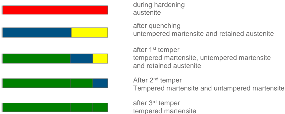
Fig. 5. Tempering of tool steel (schematic)
