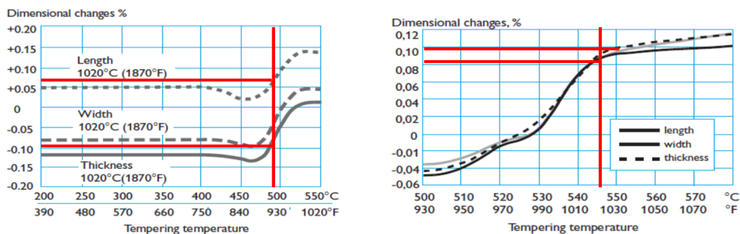
Fig. 2. Dimensional in changes conventional ingot cast steel (left), ESR and PM steels (right)
