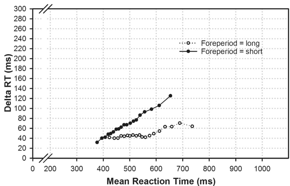
Fig. 5 Delta plots of the mobilization effect for each of the short-FP (vs. long-FP) condition. For each percentile, the RT difference between the experimental conditions (standard vs. effort) is plotted against the mean of the conditions in that percentile, comparing sequence pairings of effort with its preceding standard trials
