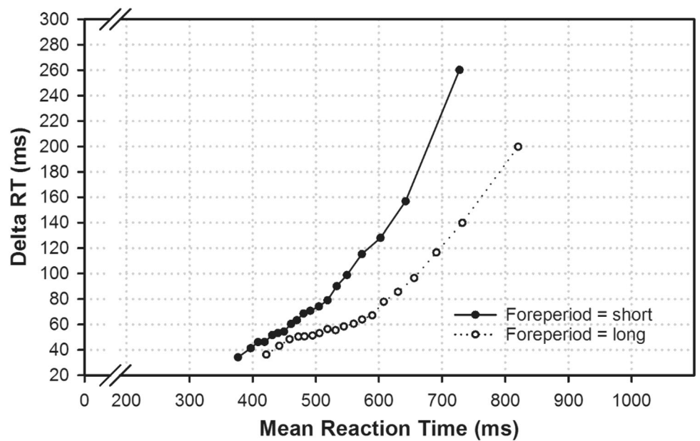
Fig. 3 Delta plots of the mobilization effect for each of the short-FP (vs. long-FP) condition. For each percentile, the RT difference between the experimental conditions (standard vs. effort) is plotted against the mean of the conditions in that percentile
