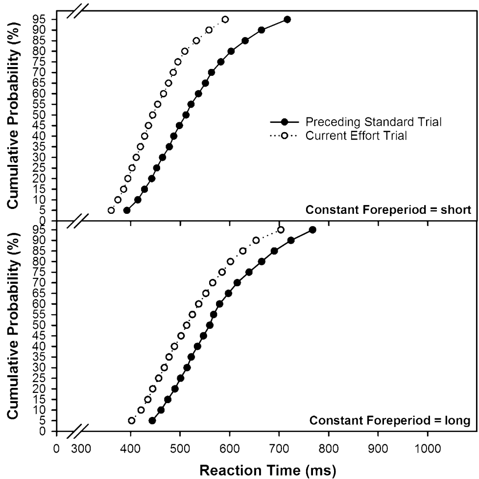
Fig. 4 Vincitized cumulative distributive function (CDFs) of reaction times for each combination of the factors foreperiod (FP: 1000 vs. 4000 ms) and the instruction to try harder (Cue: standard vs. effort), comparing sequence pairings of effort with its preceding standard trials
