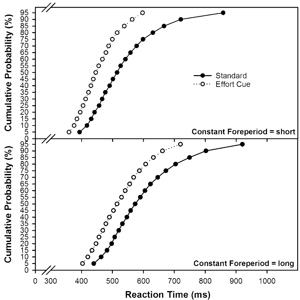
Fig. 2 Vincitized cumulative distributive function (CDFs) of reaction times for each combination of the factors foreperiod (FP: 1000 vs. 4000 ms) and the instruction to try harder (Cue: standard vs. effort)
