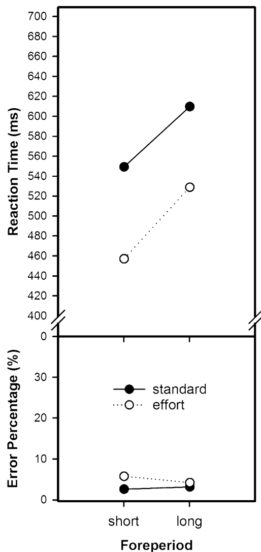
Fig. 1 Reaction time mean and error rate (RTM, EP) as a function of the factors foreperiod (FP: 1000 vs. 4000 ms) and instruction (Cue: standard vs. effort) in the speeded choice-reaction task
