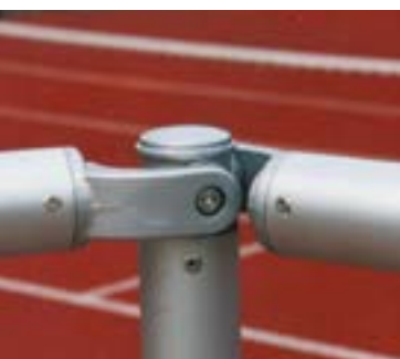
double hinge
