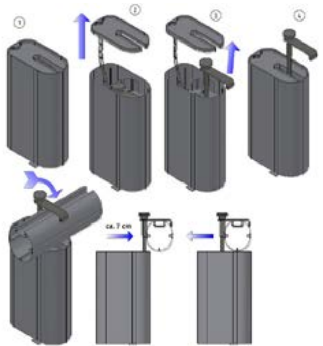
clamping ground socket 1110200 clamping ground socket
