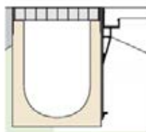
Border to a drainage gutter
