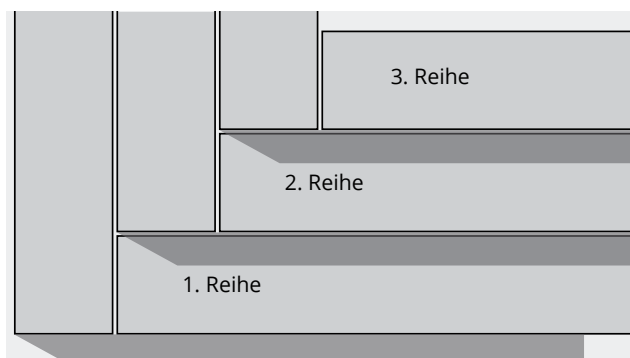
Corner 90°, with normal and finish elements
