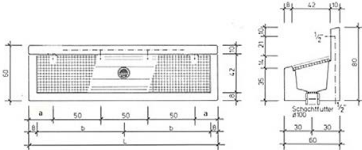
Shoe wash system „Typ D“, The raised solution with integrated back
