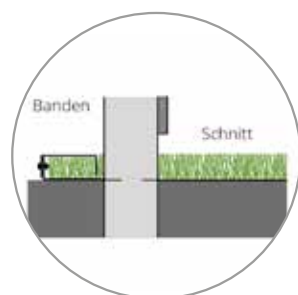
Edge/Cross section
