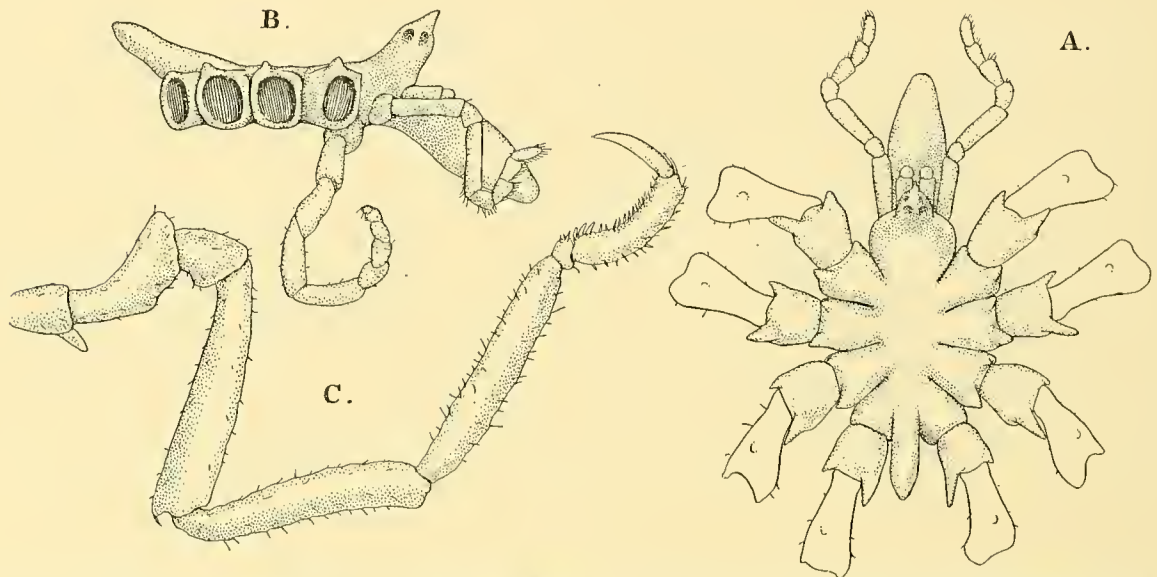
FIG. 15.— Achelua intermedia , sp. n., ovigerous Male. A. Dorsal view of body with chelophores, palps, and first and second coxæ. B. Lateral view of body with chelophore, palp, and oviger. C. Third leg of right side.
