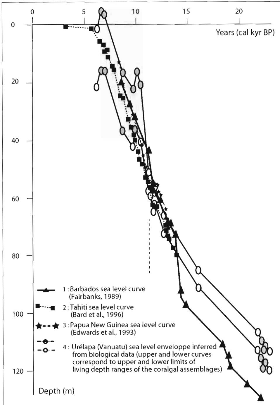
Figure 6: Deglacial sea-level curves for different reefs worldwide (modified from Cabioch, 2001).
