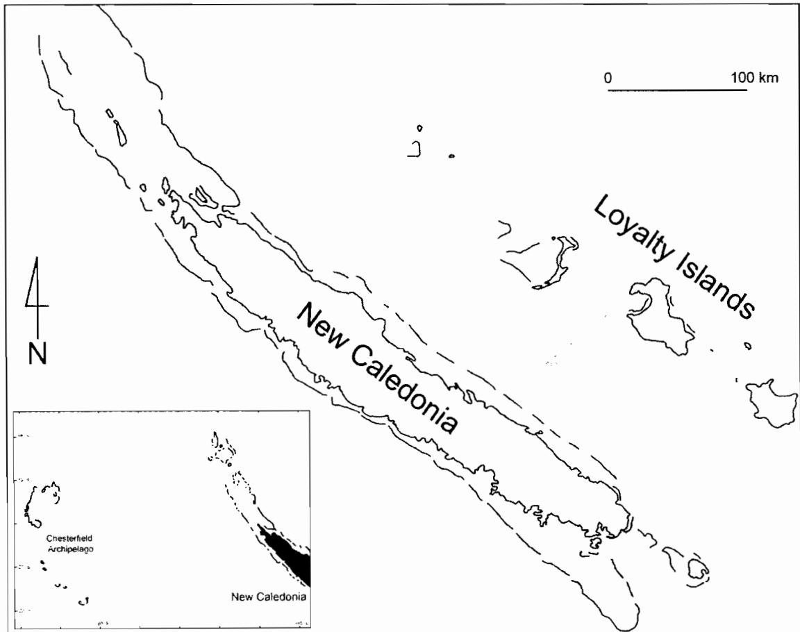
Location of the areas where foraminifera were studied (shaded areas)
