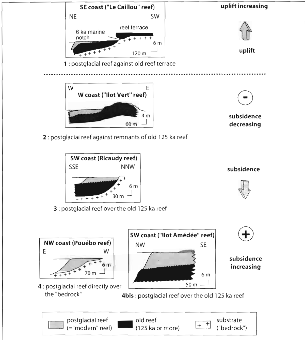
Figure 4: Morphology and structure of reefs depending on tectonic forcing (modified from Cabioch et al. 1999, Cabioch 2003).
