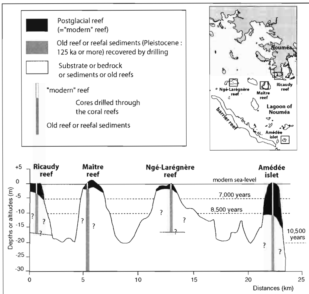
Figure 5: Relationships between the timing of the flooding and available substrates and age of the coral reef formations of the Nouméa lagoon inferred from core data (modified from Castellaro et al. 1999, Cabioch et al. 1999 and unpublished data)
