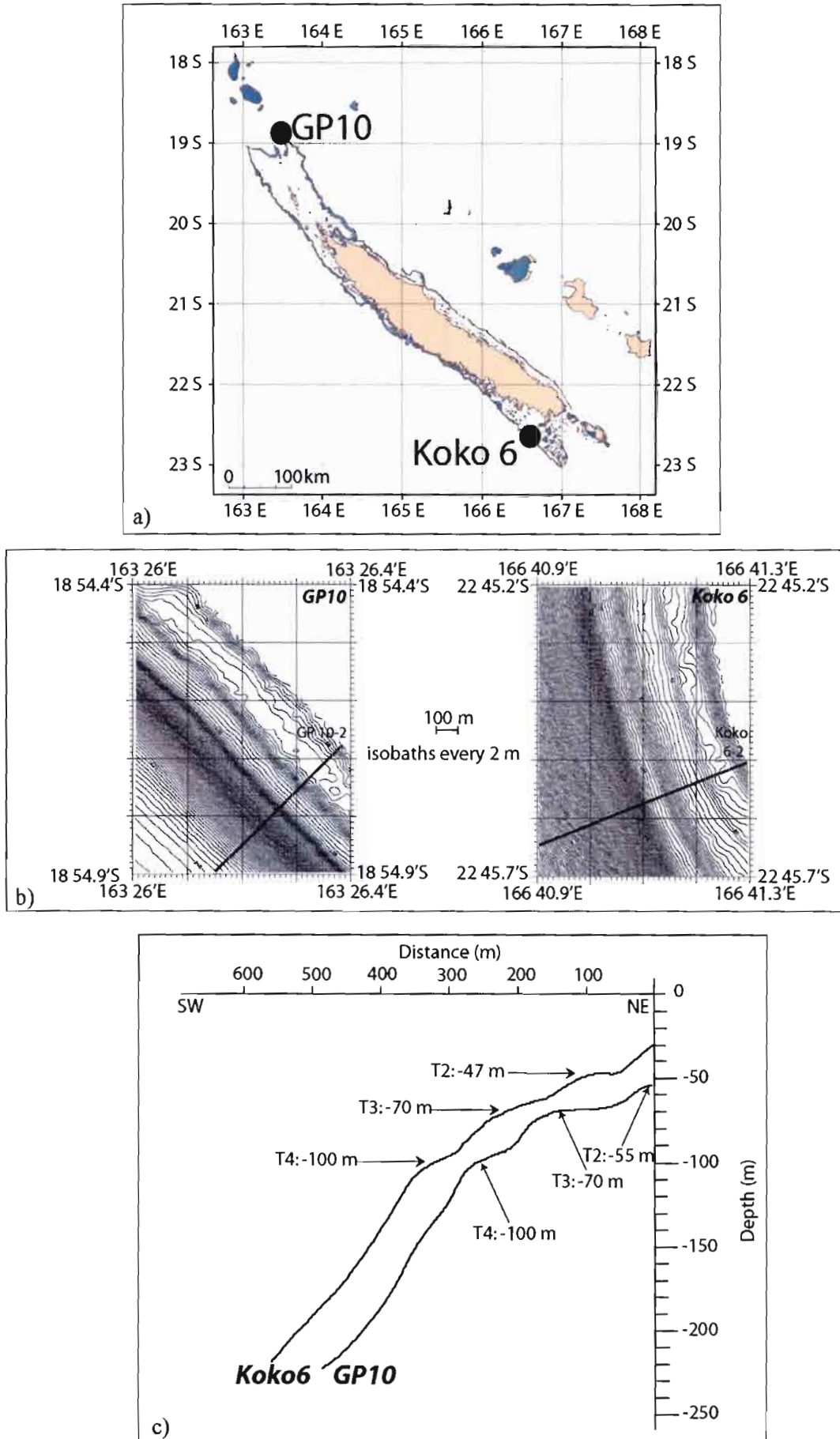
Figure 9. Detailed bathymetric maps from two different locations, in the north (Grand Passage 10) and South (Koko 6) of New Caledonia. The profiles show the depth and morphology of the marine terraces.
