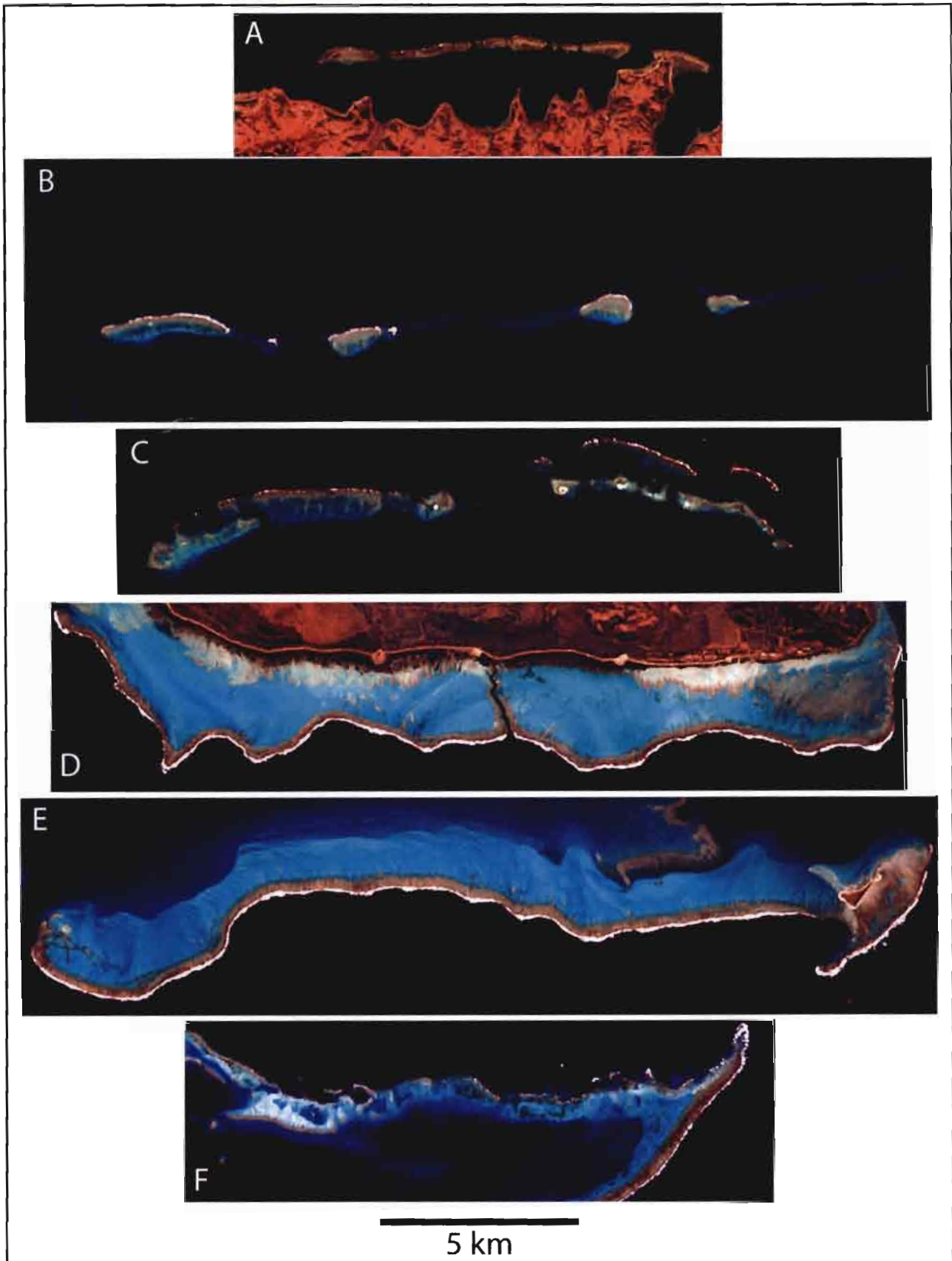
Figure 8. Examples of the diversity of New Caledonia barrier reefs (BR). Landsat images acquired between 1999-2003. Images are at the same scale, but have been rotated for easier comparisons.
