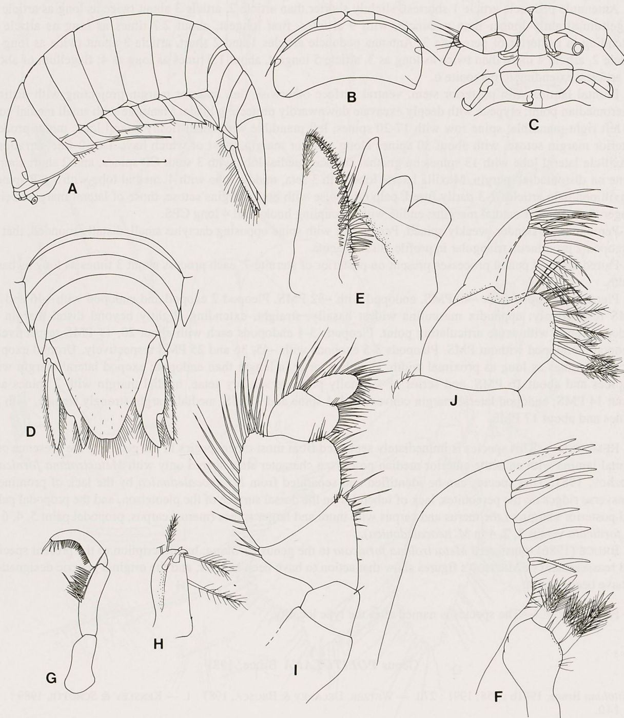
FIG. 10. — Politolana crosnieri sp. nov. A , lateral view; B , cephalon, dorsal view; C , frons; D , pleon and pleotelson, dorsal view; E , right mandible; F , maxillule; G , mandible palp; H , maxilliped endite; I , maxilliped; J , maxilla. A , scale 3.0 mm.
