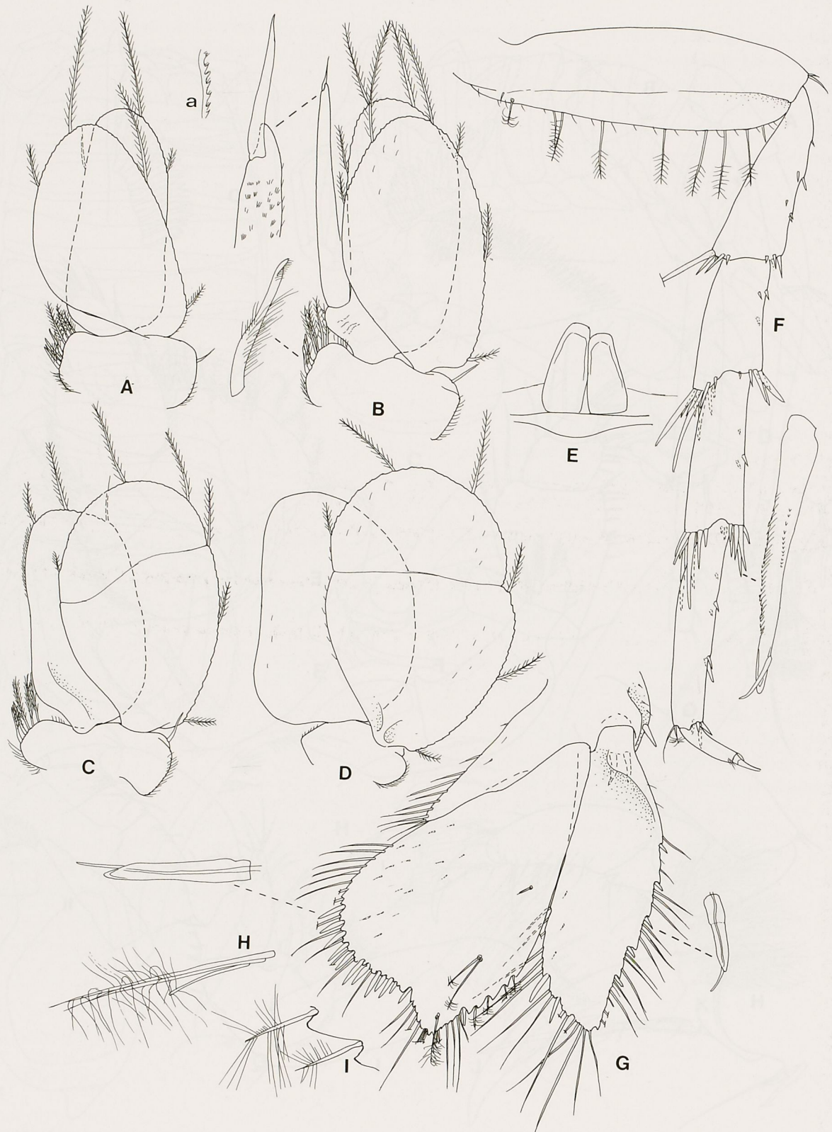
FIG. 9. — Metacirolana neocaledonica sp. nov. Holotype, except F. A-D , pleopods 1-3 and 5 respectively, a , detail of endopod proximolateral margin; E , penes, in situ; F , pereopod 7; G , uropod; H , setae from distolateral surface of uropod endopod; I , setae from lateral margin of uropod endopod.
