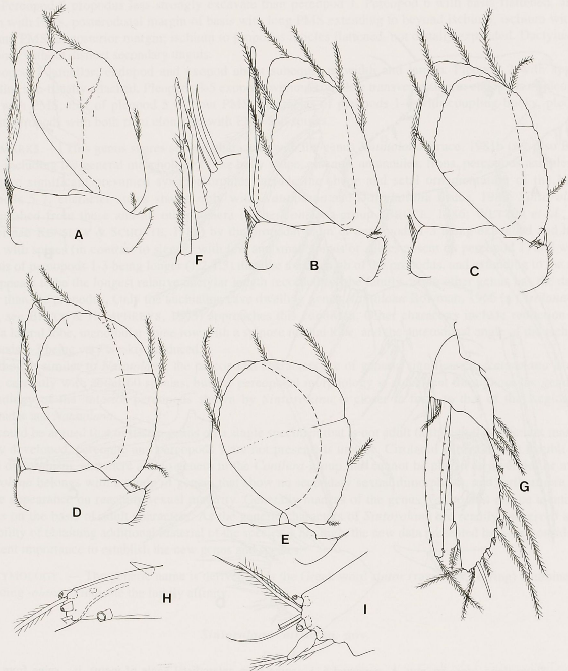
FIG. 6. — Sintonrolana atrox sp. nov. A-E, pleopods 1-5 respectively; F, coupling hooks, medial margin pleopod 1; G, uropod, ventral view; H, uropod exopod, apex; I, uropod endopod, apex.
