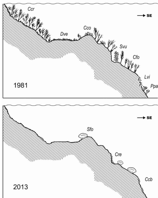
Fig. 12: Schematic profile of a reef slope down to about 7 m depth at site N, to illustrate change between 1981 and 2013. Species codes as in Table 1.
