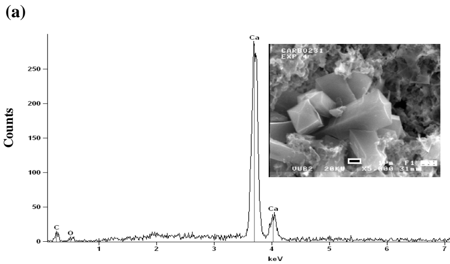
Fig. 3. (a) Energy dispersive x-ray (EDX) analysis of prismatic and bipyramidal crystals (inserted figure) showing high calcium content with C and O. These biomineralized crystals making the fine background proved to be composed of Ca-oxalates: weddellite and whewellite.
