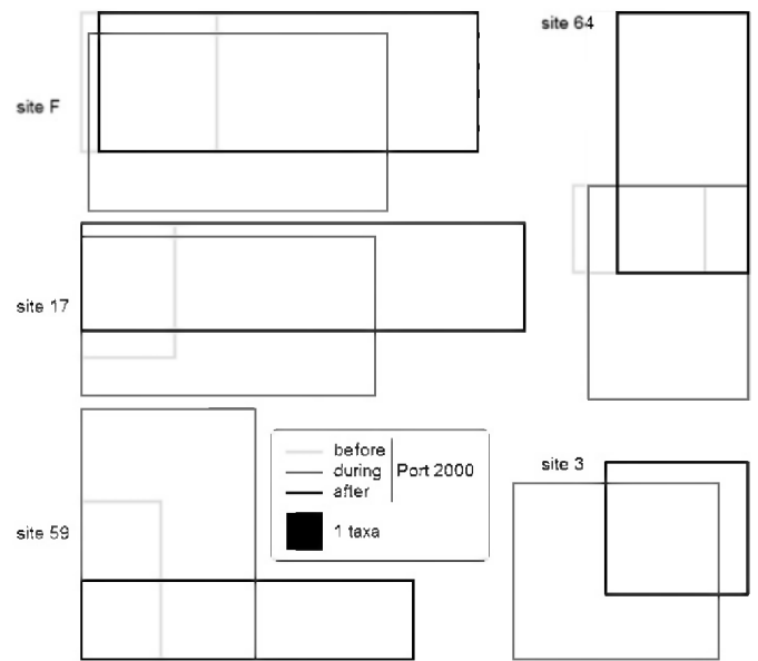
Fig. 4. Number of common taxa for the five sites for the three periods: Before/During/After Port 2000 construction.
