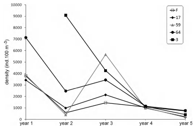
Fig. 5. Temporal changes of the total density of the suprabenthic fauna (number of individuals per 100\text{ m}^{-3} ) for all five years of observations at all five sites in the North Channel of the Seine estuary.
