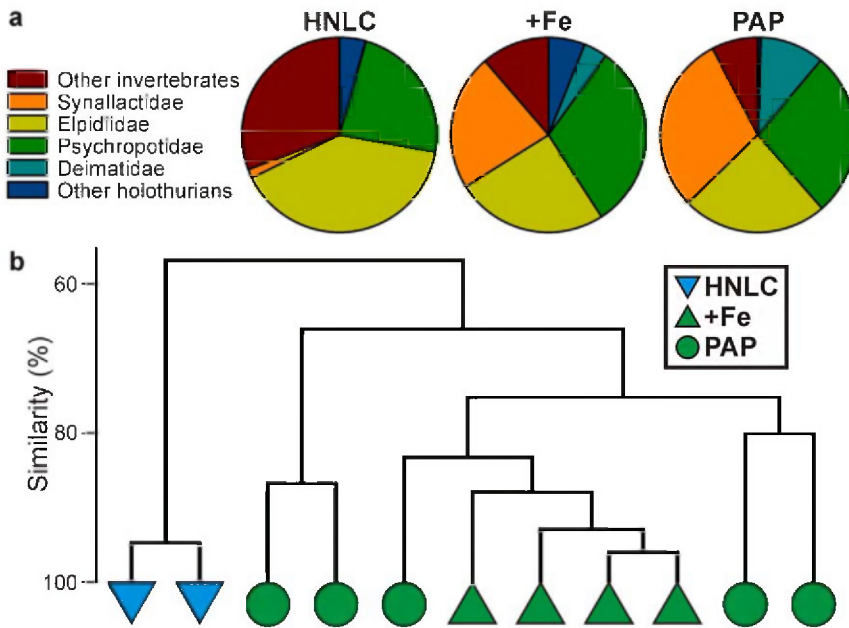
Figure 6. Fresh wet weight biomass composition of the megabenthos at Crozet (HNLC, +Fe) and the NE Atlantic Porcupine Abyssal Plain (PAP) sites. A. Average relative biomass of dominant holothurian families, combined ‘other holothurians’ and ‘other invertebrates’. B. Similarity of individual trawl catches based on the relative biomass of the same taxonomic groups (proportional biomass; Bray-Curtis similarity; group-average clustering). doi:10.1371/journal.pone.0020697.g006
