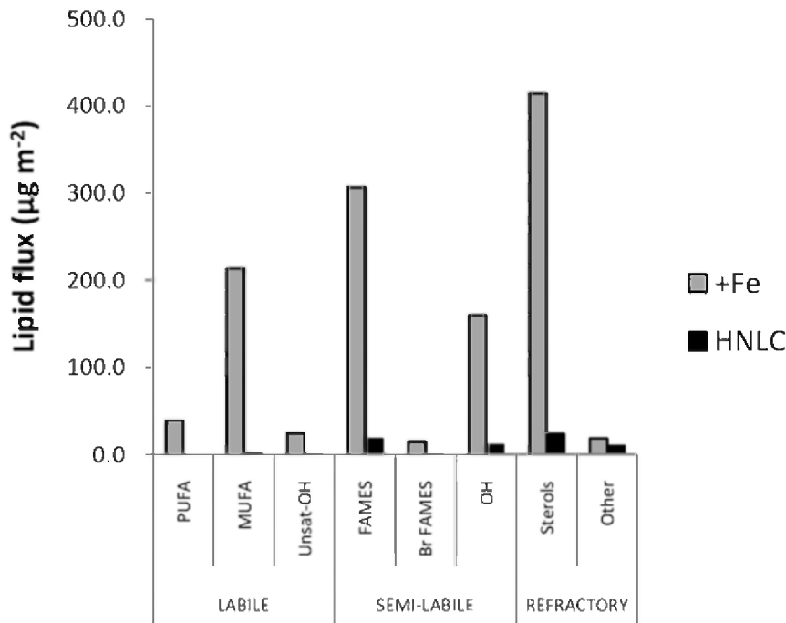
Figure 3. Lipid fluxes at the Crozet abyssal locations, +Fe and HNLC at 3195 and 3183 m water depth in 2005. Labile lipids: Polyunsaturated fatty acids (PUFA), monounsaturated fatty acids (MUFA) and unsaturated alkanols (U-ALK); Semi-labile lipids: Saturated fatty acids (FA), branched fatty acids (Br-FA) and n -alkanols (ALK); Refractory lipids: Sterols (STER) and other lipids including branched alkanols, triterpenoids, steroidal ketones, phytol derivatives and alkenones (OLIP). doi:10.1371/journal.pone.0020697.g003
