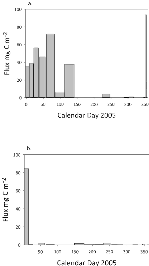
Figure 2. Carbon fluxes determined over a period of ~12 months in 2005 at the Crozet Plateau (see also Ref. 12): a. the +Fe site at 3183 m water depth b. the HNLC site at 3195 m water depth. Both ~1000 m above the seabed. Bar widths are proportional to cup opening times of the Parflux sediment traps. Bar heights represent the material supplied over the period of cup opening. doi:10.1371/journal.pone.0020697.g002
