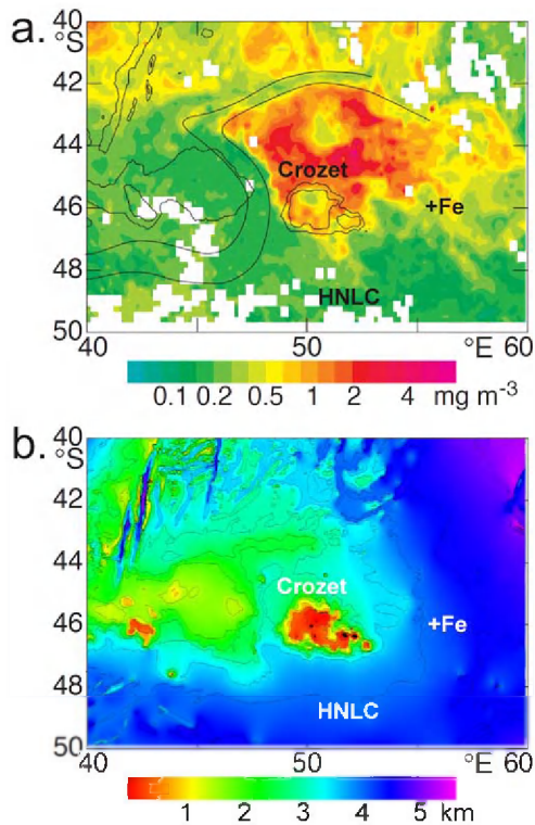
Figure 1. Location maps of the +Fe and HNLC sites with respect to: a. monthly (October 1998) SeaWiFS chlorophyll ( \text{mg m}^{-3} ) distribution, showing a typical spring bloom to the north of the Crozet Plateau (adapted from Ref. 15), with the meander of the Sub-Antarctic Front indicated by parallel black lines. b. Water depth (km) in the corresponding Crozet region (derived from the General Bathymetric Chart of the Oceans, Centenary Edition). doi:10.1371/journal.pone.0020697.g001
