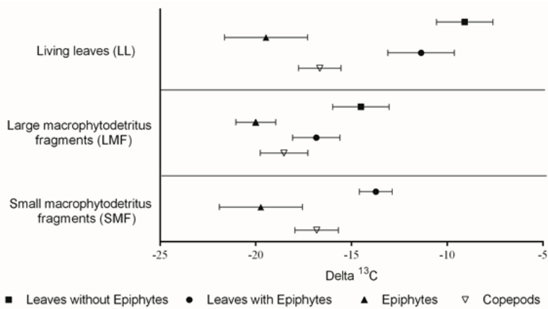
Fig. 5 \delta^{13}C values (‰) of plant material as potential food sources and copepods (mean \pm SD, n=3). The full symbols are potential sources: leaves (living or macrophytodebris) without epiphytes (squares), the removed epiphytes (triangles) and the leaves (living or macrophytodebris) with their epiphytes (rounds). The open symbols are the harpacticoid copepods, primary consumers (reversed triangles).
