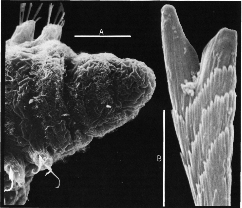
Fig. 2. Gymnodorvillea floridana , paratypes: A, Anterior region, dorsal view, showing ciliary bands, shrinkage due to fixation and/or critical-point drying; B, Furcate seta (SEM photomicrographs). Scales: A = 50 \mu\text{m} , B = 5 \mu\text{m} .
