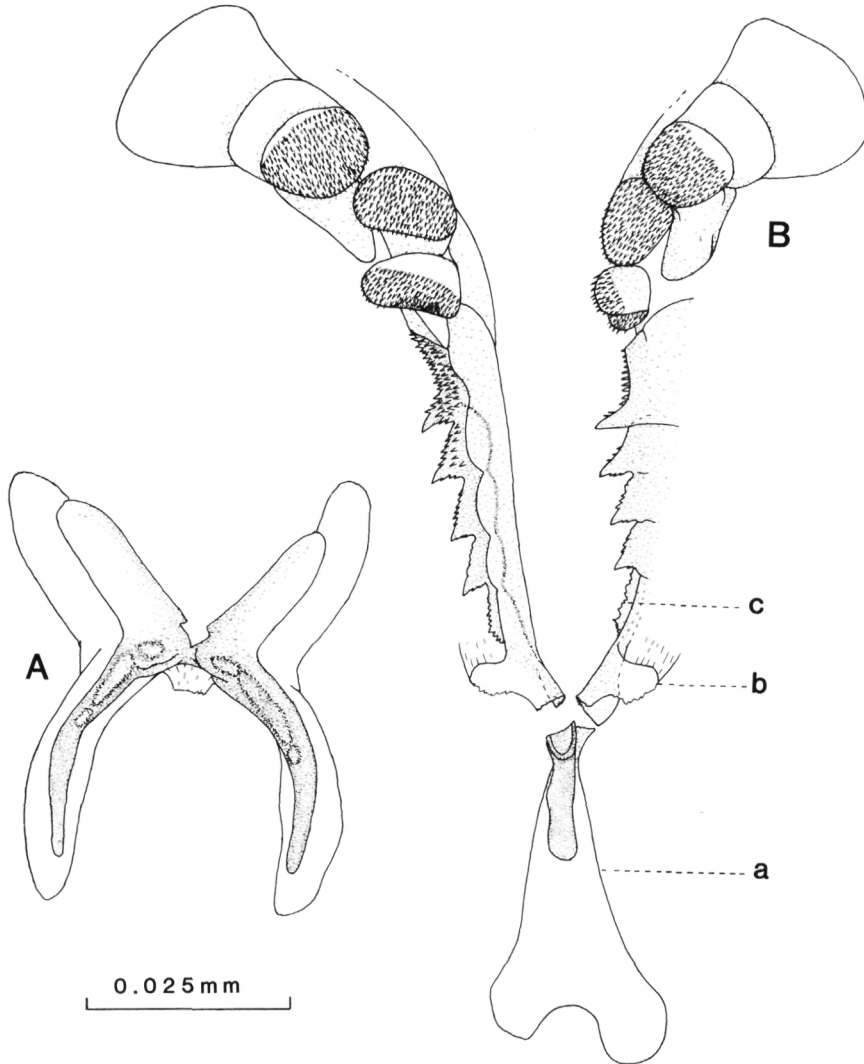
Fig. 3. Gymnodorvillea floridana , paratypes: A, Mandibles, dorsal view; B, Maxillae, denticles 1-6 turned, posterior maxillary piece broken, a, posterior tonguelike extension of maxillary ligament, b, winglike projection on basal piece, c, posterior denticle.
