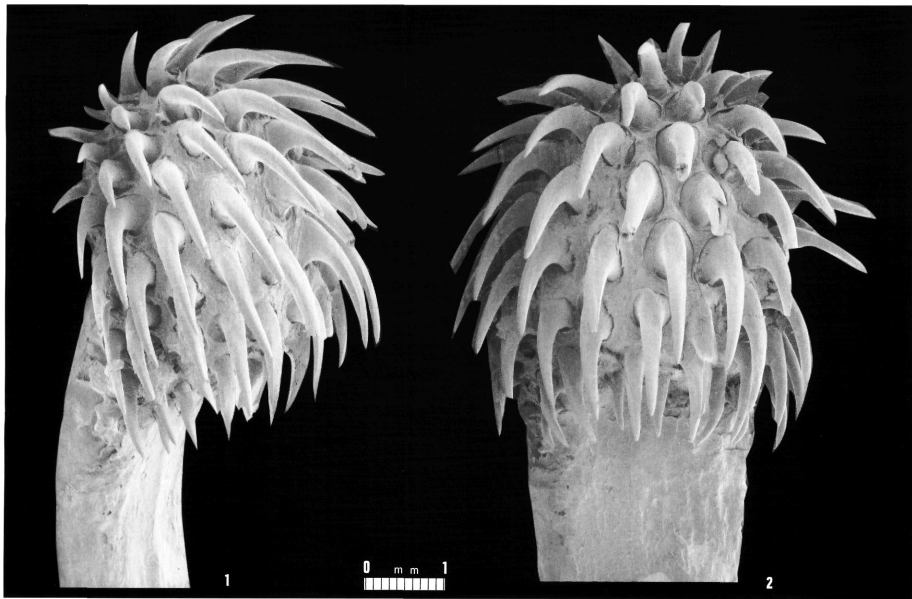
Plate 11. Hydrolagus mirabilis (COLLETT, 1904). Male circa 75 cm t.l., no precise locality data, «North East Atlantic». Right lateral (fig.1) and front (fig.2) views of the frontal tenaculum head.
