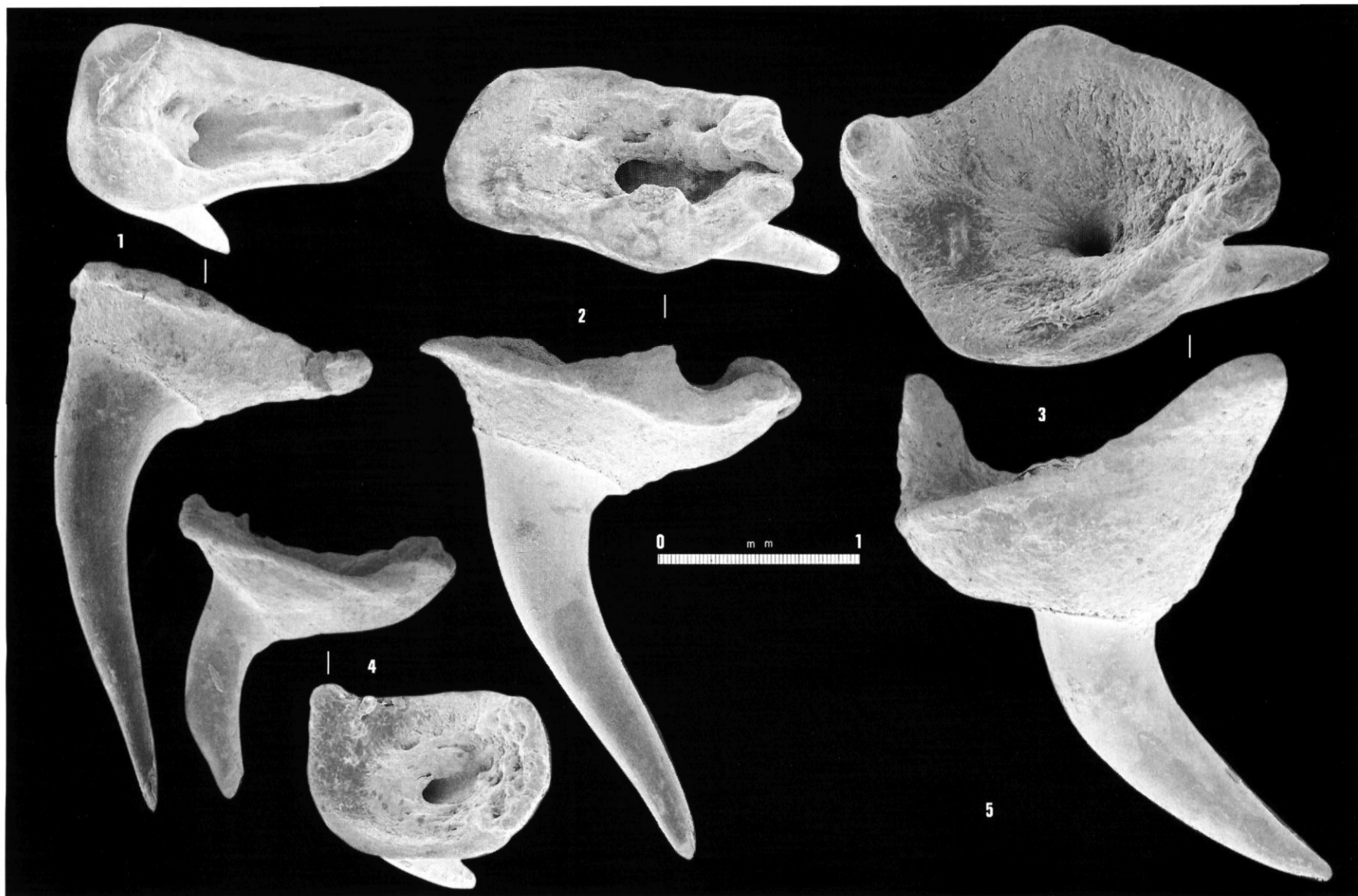
Plate 19. Rhinochimaera atlantica HOLT & BYRNE, 1909. Male circa 105 cm t.l., Hatton Bank North East Atlantic. Basal or radicular and lateral views of some of the tooth-like dermal denticles of the frontal tenaculum head.
