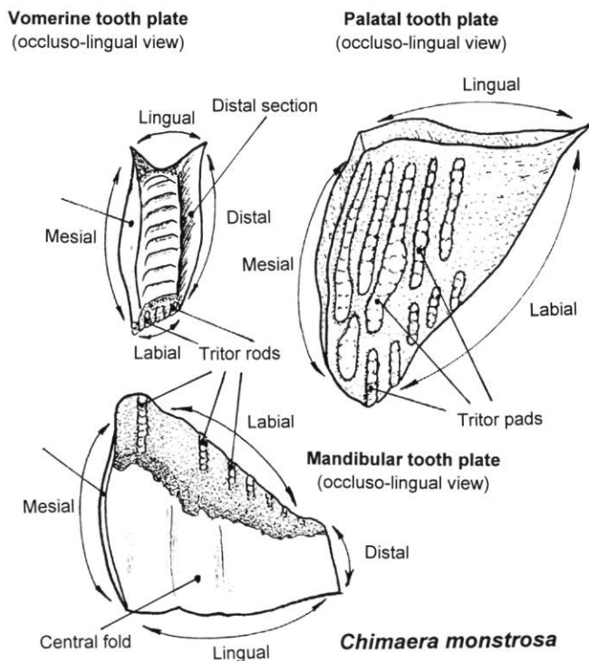
Text figure 1 – Description of the odontological spine of the first dorsal fin and tenaculum characters
