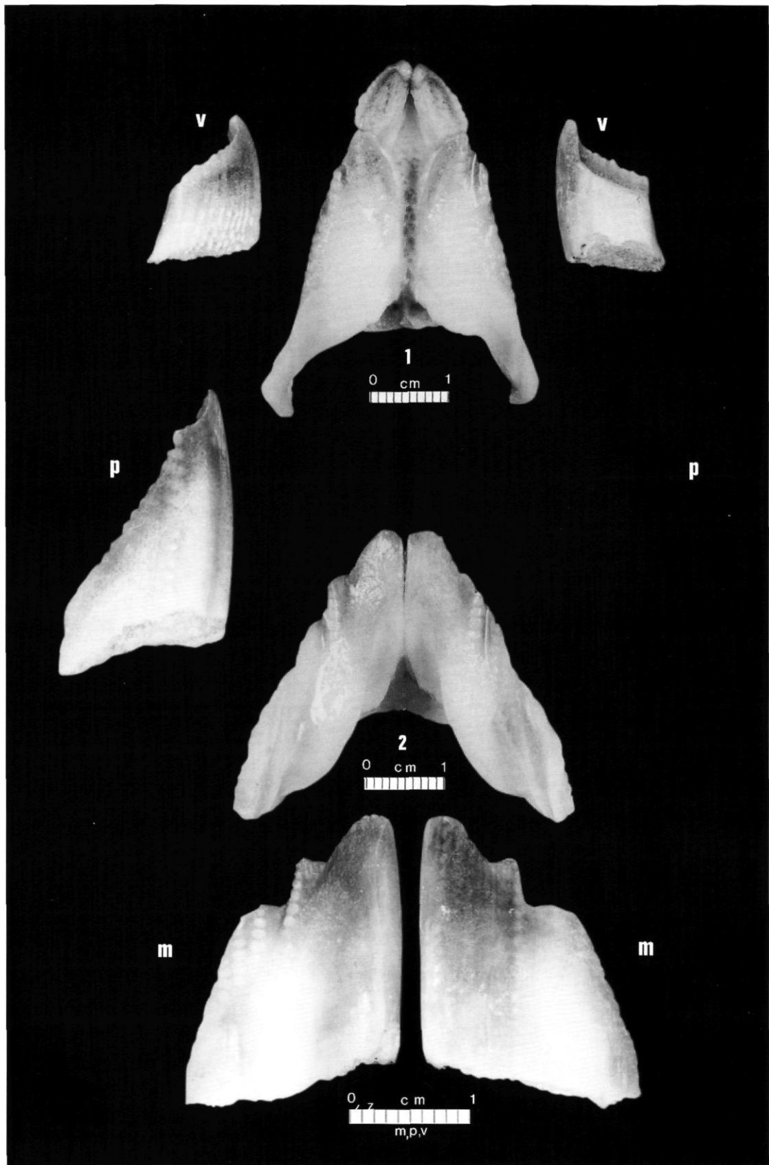
Plate 13. Haviotta raleighana GOODE & BEAN, 1895. Female circa 90 cm t.l., no precise locality data, "North East Atlantic". Inner view of upper (fig.1) and lower jaws (fig.2). Lingual (functional) and labial views of the three left dental plates ( v , p , m ).
