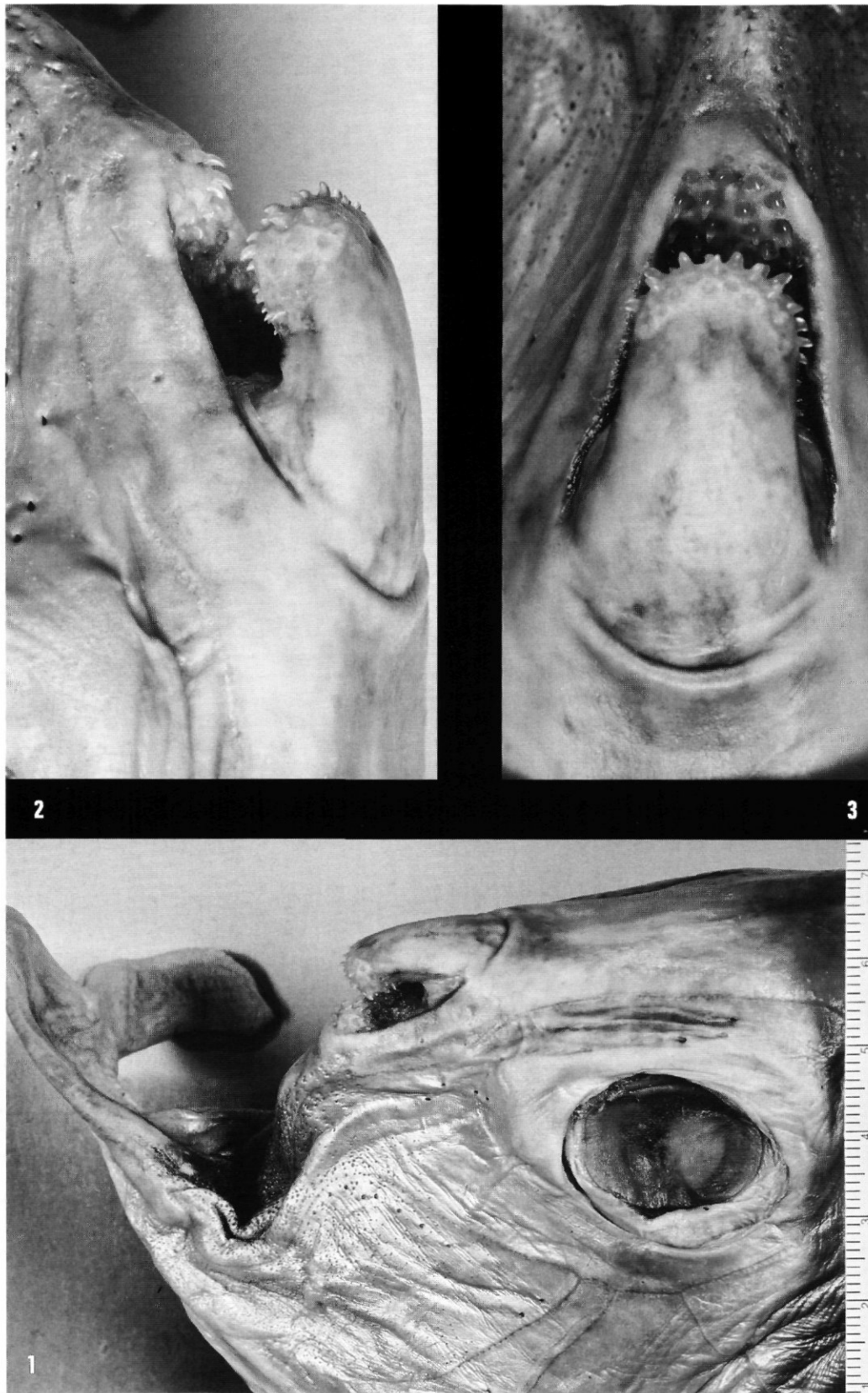
Plate 1. Callorhynchus milii BORY & SAINT VINCENT, 1823. Male, 78 cm t.l., off south east Australia, IRSNB, R. 3455, collected in 1874. Fig.1: partial left lateral view of the head ; details of the frontal tenaculum complex : lateral view (fig.2) and dorsal view (fig.3).
