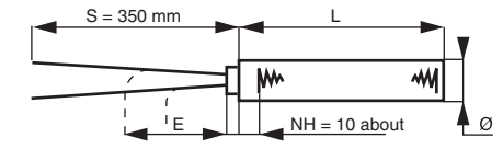
Model without Thermocouple (TC K/J)
