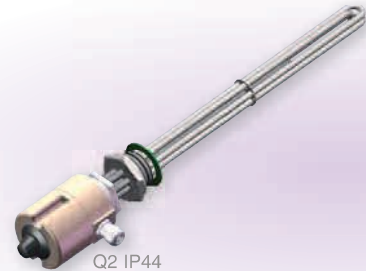
Q2 IP44 P/n. 2216-xx P/n. 3216-xx Control thermostat -20/+40°C P/n. 9030-71 External setting button
