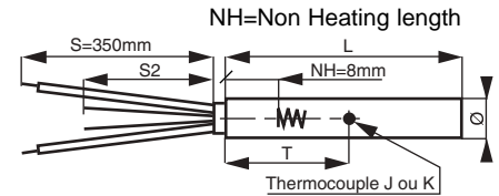
Model with Thermocouple (TC K/J)
