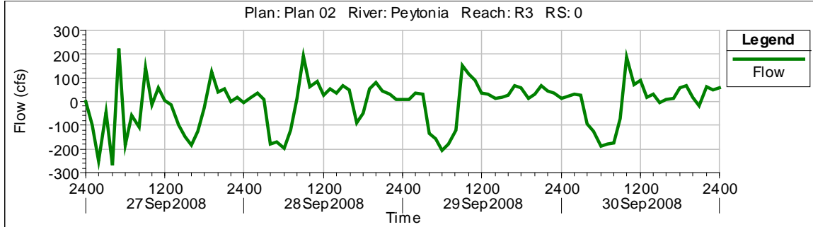
Figure C-15 Simulated variations in flow near the mouth of Peytonia Slough (R3, 0.0 km from mouth) by HEC-RAS
