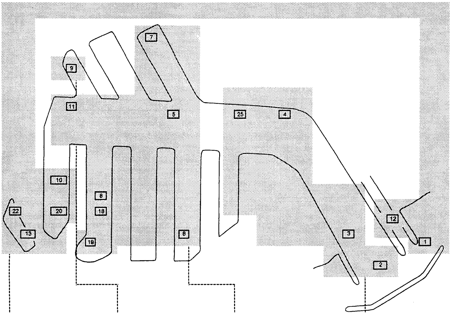
FIGURE 3-34. WATER QUALITY CHARACTERISTICS BASED ON BRAY-CURTIS CLUSTERING TECHNIQUE.
