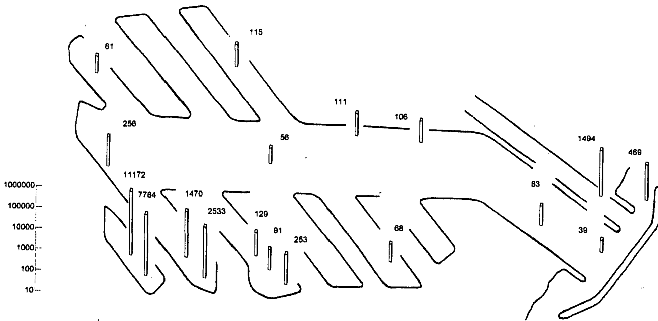
FIGURE 3-29. GEOMETRIC MEANS OF TOT. COLIFORM (MPN/100 ML) AT 18 WATER COLUMN STATIONS.
