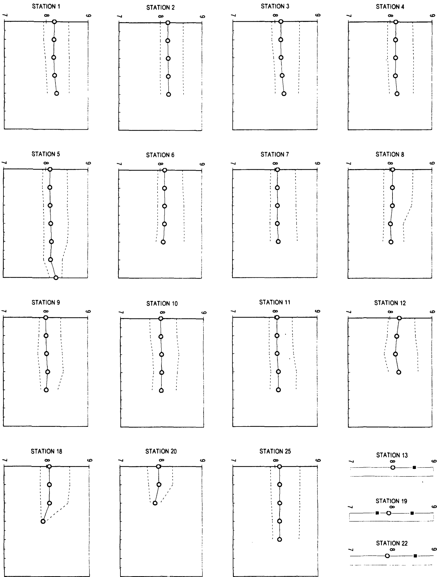
FIGURE 3-12. MIN, AVERAGE, AND MAX PH (UNITS) VERSUS DEPTH (M) AT 18 WATER COLUMN STATIONS.
