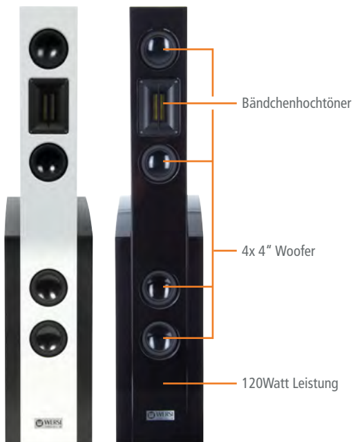
WERSI Vocalis
